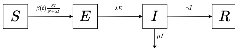
Fig. 2: SEIR model diagram
