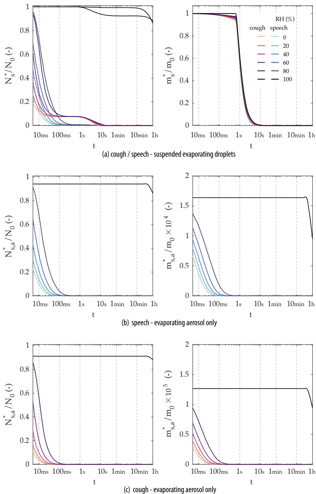
Figure 7. Time evolution of ensemble quantities (total mass and number) normalised by the respective value at t = 0 for sprays exhaled by speech and cough – T=20^{\circ}\text{C} , \text{RH}=0\text{--}100\% . The quantities only consider evaporating droplets, that is, droplets that have not yet achieved equilibrium with ambient air. In the lower row, ensemble quantities shown are calculated considering only droplets below 5\ \mu\text{m} .
