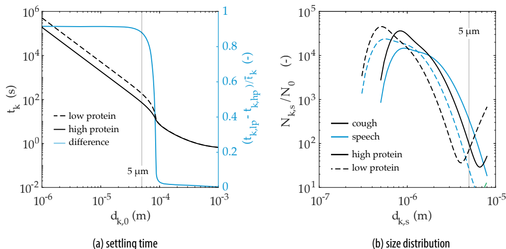
Figure 9. (a) Settling time (left axis) and its respective relative difference (right axis) of droplets and (b) probability density functions of droplet size normalised by the initial number of droplets at t = 10 min for coughing and speaking, both presented in terms of the saliva composition: low protein (sputum 9 mg/ml NaCl, 3 mg/ml protein) and high protein (sputum 9 mg/ml NaCl, 76 mg/ml protein) – T=20^\circ\text{C} , \text{RH}=80\% .
