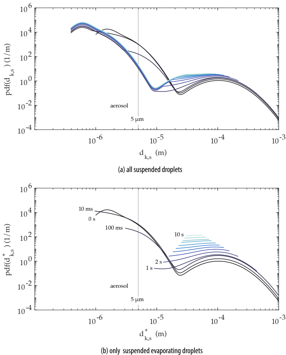
Figure 3. Evolution of the probability density function of droplet size from speaking for various times after droplets are exhaled. In (a) all suspended droplets are considered, and (b) only droplets that have not yet reached equilibrium – T=20^\circ\text{C} , \text{RH}=80\% .
