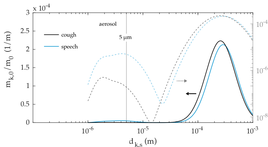
Figure 4. Initial mass in each droplet size category normalised by the total emitted mass of sputum in coughing and speaking. Dark lines represent the curves plotted in a linear vertical scale (left side y-axis), while the lighter colours represent the curves plotted in a vertical log scale (right side y-axis).
