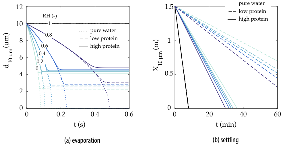
Figure 8. Impact of the droplet composition modelling approach (pure water; sputum 9 mg/ml NaCl, 3 mg/ml protein; sputum 9 mg/ml NaCl, 76 mg/ml protein) on the (a) evaporation and (b) settling of 10 μm droplets under different relative humidities. The relative humidity is shown in colour (RH=0–100%) – T=20°C.
