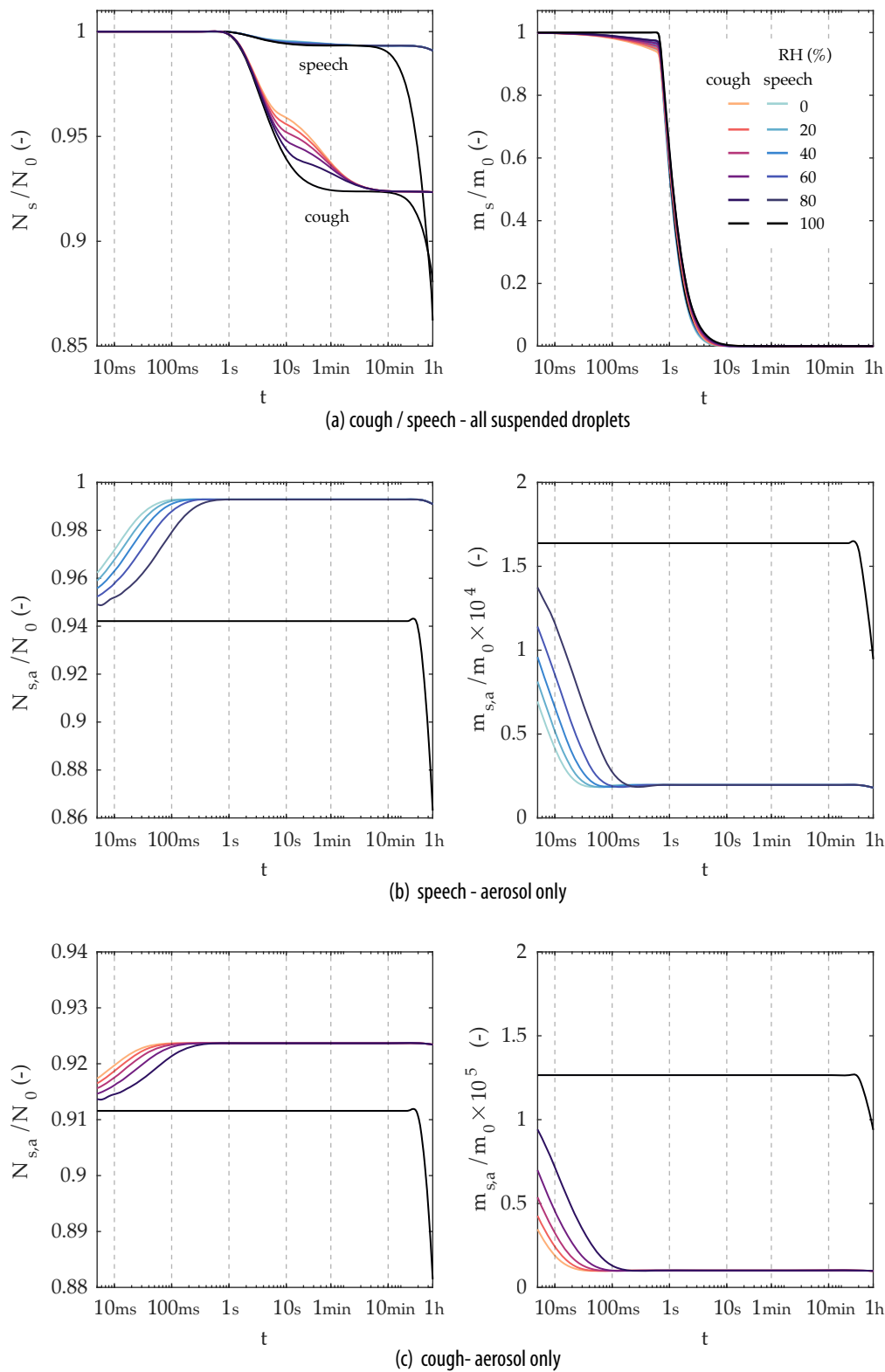
Figure 5. Time evolution of ensemble quantities (total mass and number) normalised by the respective value at t = 0 for sprays exhaled by speech and cough – T=20^{\circ}\text{C} , \text{RH}=0\text{--}100\% . In the top row, ensemble quantities shown are evaluated for all suspended droplets, while in the middle and lower low the quantities are calculated considering only droplets below 5\ \mu\text{m} . More detail on the time evolution of m_s/m_0 is provided in Fig. 6.
