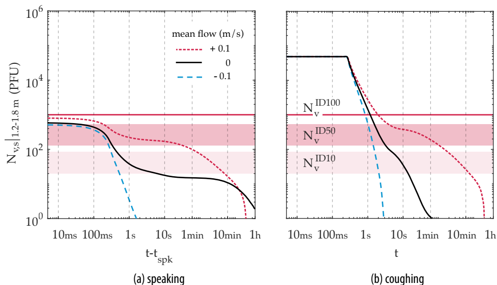
Figure 12. Evolution of the suspended viral dose at face height (between 1.2–1.8 m) following 30-s continuous speech and a short cough (i.e. same exhaled liquid mass) for three cases of ambient mean flow: upward (+0.1 m/s), zero, downward (-0.1 m/s) – low-protein sputum, RH=40%, n_{v,0} = 10^9 copies/ml).
