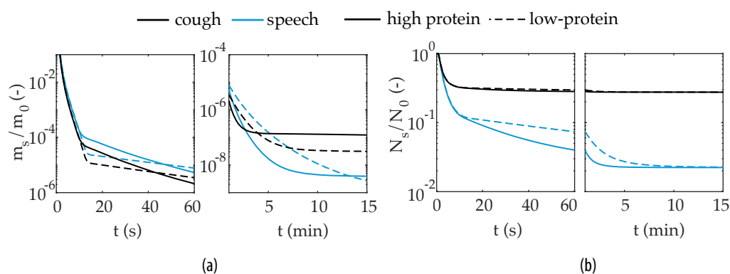
Figure 10. Time evolution of (a) total mass and (b) total droplet number, all normalised by their respective values at t = 0 , in terms of the composition: low protein (sputum 9 mg/ml NaCl, 3 mg/ml protein) and high protein (sputum 9 mg/ml NaCl, 76 mg/ml protein) – T=20^\circ\text{C} , \text{RH}=80\% .
