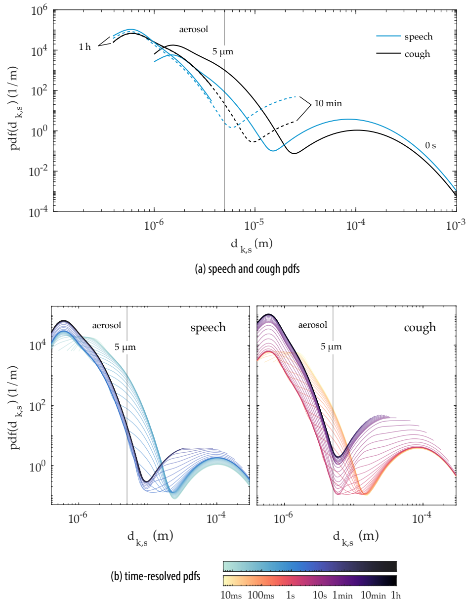
Figure 2. Evolution of the probability density function of droplet size from speaking and coughing, where (a) shows 0 s, 10 min, and 1 h pdfs, and (b) shows detailed time-resolved pdfs between 0–1 h coloured in a log scale – T=20^{\circ}\text{C} , \text{RH}=80\% .
