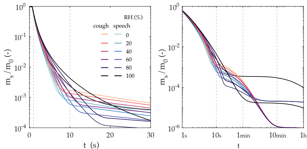
Figure 6. Detail of the time evolution of total mass normalised by the respective value at t = 0 shown in Fig. 5. The left-hand side plot is given in a linear time scale up to 30 s, while the right-hand plot is given for a log scale up to 1 h.
