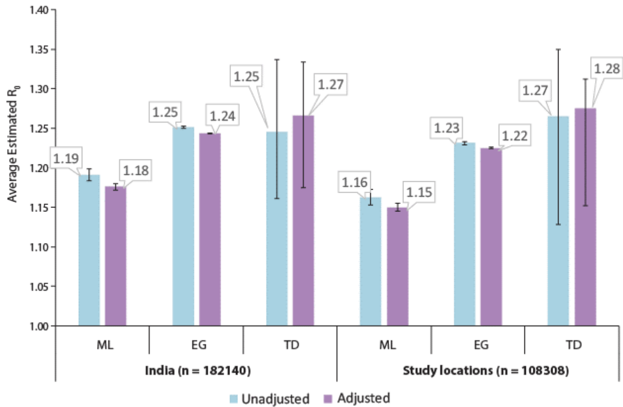
436 Figure 2. Average estimated R_0 for COVID-19. Bars show the average R_0 estimates and error 437 bars indicate the 95% confidence intervals. Average R_0 estimates were derived using three 438 methods: ML, maximum likelihood; EG, exponential growth; and TD, time dependent. Each 439 estimate was also derived without adjustment (unadjusted, blue bars) and adjusted for potential 440 undertesting (adjusted, purple bars).
