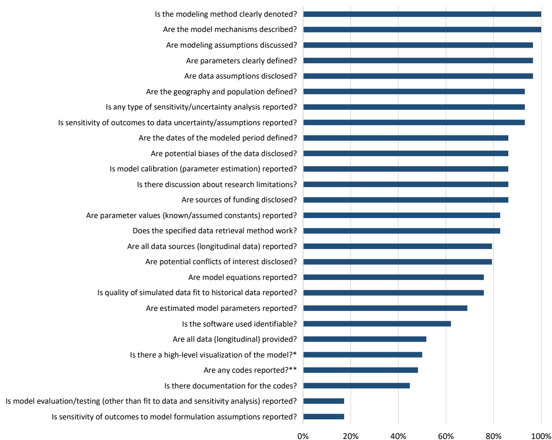
Fig. 1. Percent of COVID-19 models (n=29) which satisfy transparency assessment criteria
