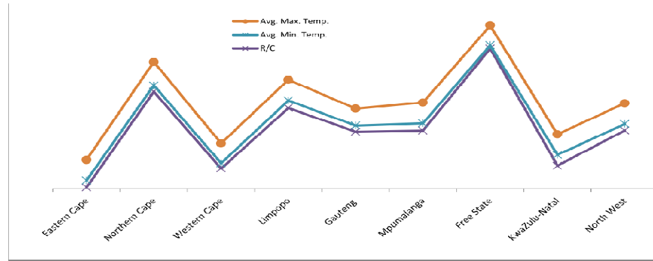
Fig. 3: Average minimum and maximum climate temperatures and recovery-to-count (R/C) for the lockdown period.
