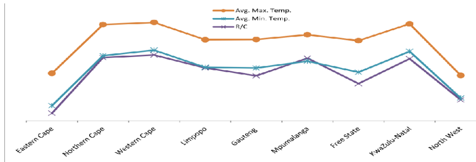
Fig. 4: Average minimum and maximum climate temperatures and recovery-to-count (R/C) for the eased-lockdown period.
