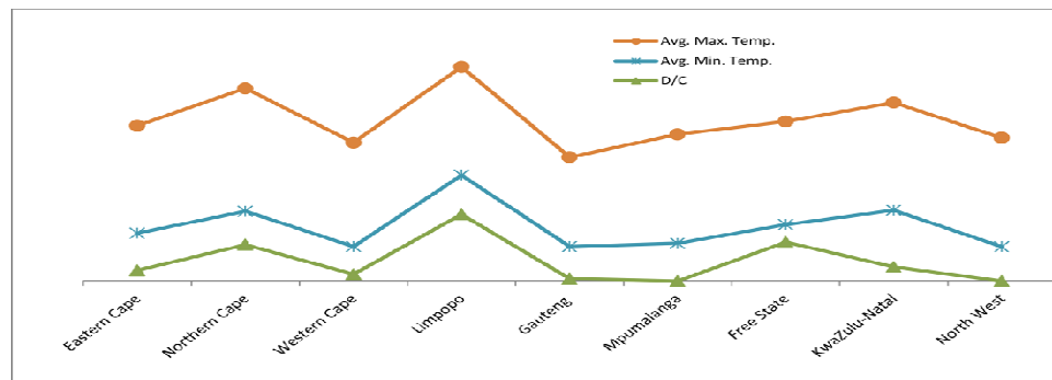
Fig. 2: Average minimum and maximum climate temperatures and death-to-count (D/C) ratio for the lockdown period.
