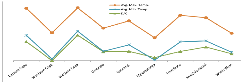
Fig. 3: Average minimum and maximum climate temperatures and death-to-count (D/C) ratio for the eased-lockdown period.
