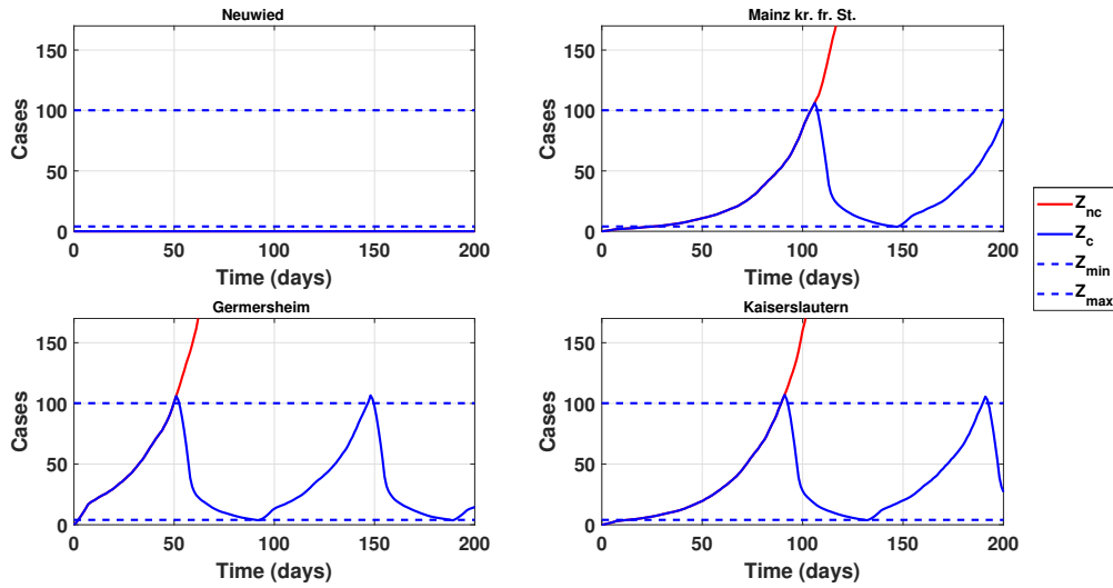
Figure 3: Controlled and uncontrolled disease progression for four districts of Rhineland-Palatinate without mobility between the districts, with Z_{\min} = 4 and Z_{\max} = 100 .
