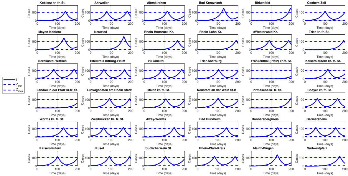
Figure 4: A sample path for the infected number of cases per 100,000 inhabitant with the optimized values obtained for the upper bound and lower bound, Z_{\max} = 100 and Z_{\min} = 4 .
