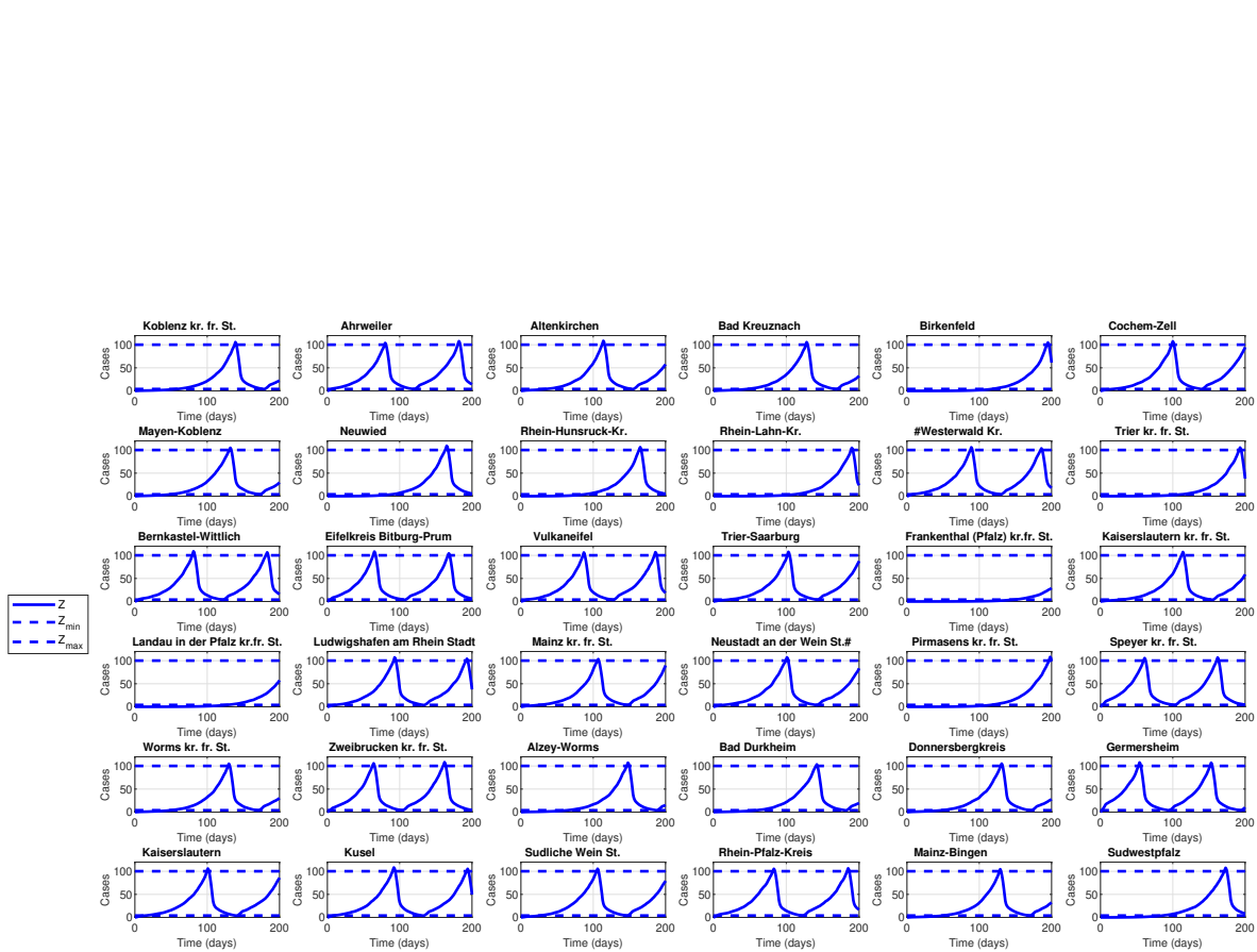
Figure 5: Number of newly infected over a 7 days timespan with controlled disease progression for Z_{\max} = 100 and Z_{\min} = 4 .
