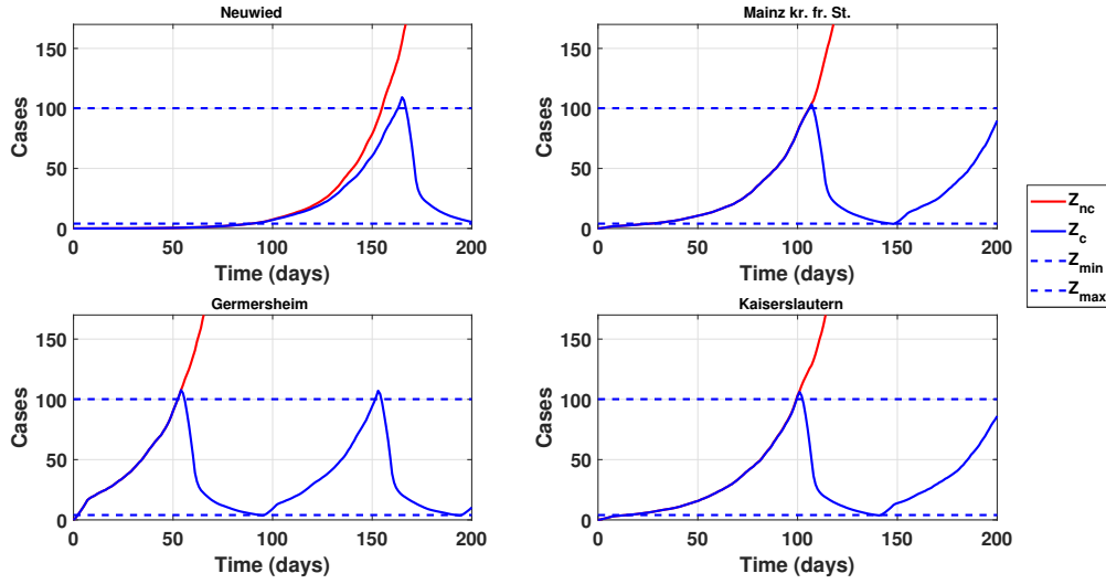
Figure 2: Controlled and uncontrolled disease progression for four districts of Rhineland-Palatinate including mobility between the districts, with Z_{\min} = 4 and Z_{\max} = 100 .
