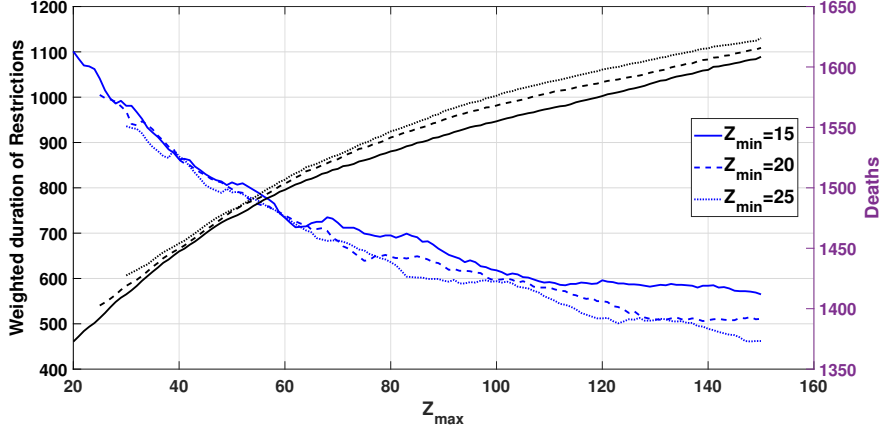
Figure 1: Weighted duration of restrictions in man-days (blue) and deaths (black) as a function of Z_{\max} and Z_{\min} for whole Rhineland-Palatinate. The different line styles indicate the lower bound Z_{\min} = 15 (solid), 20 (dashed) or 25 (dotted).
