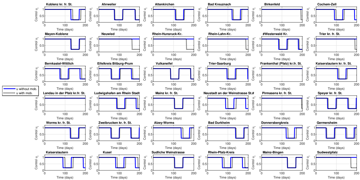
Figure 6: Time dependent control for for Z_{\max} = 100 and Z_{\min} = 4 .
