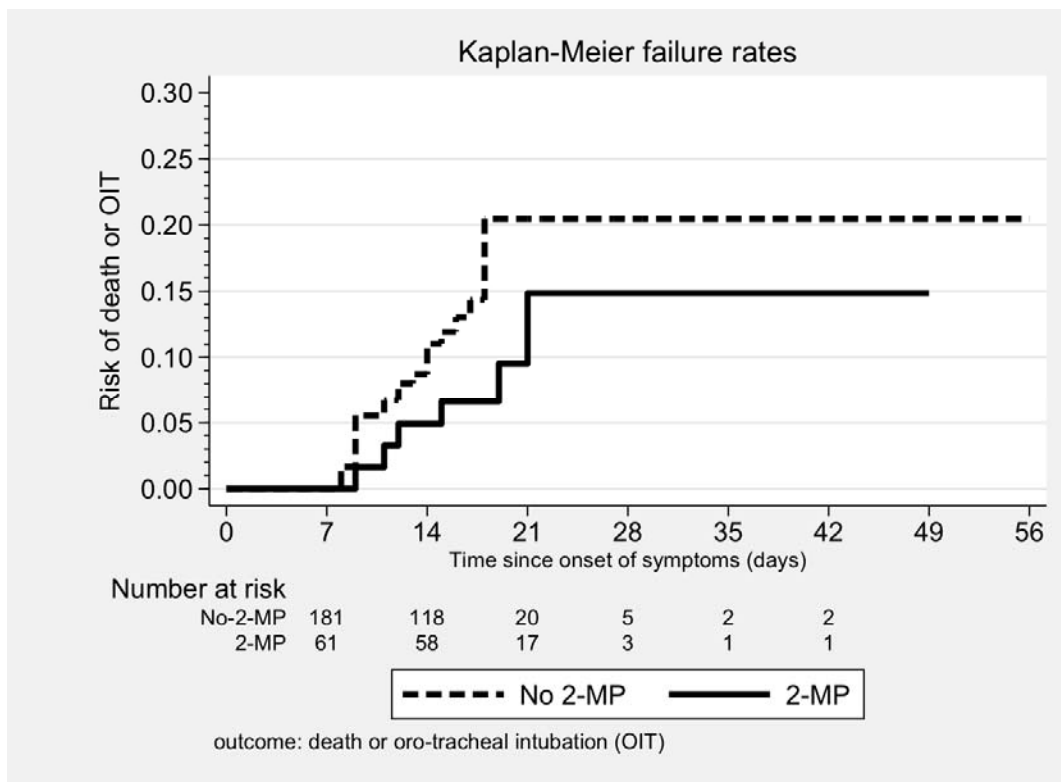
Figure 2. Kaplan-Meier failure curves. Outcome: death or intubation
