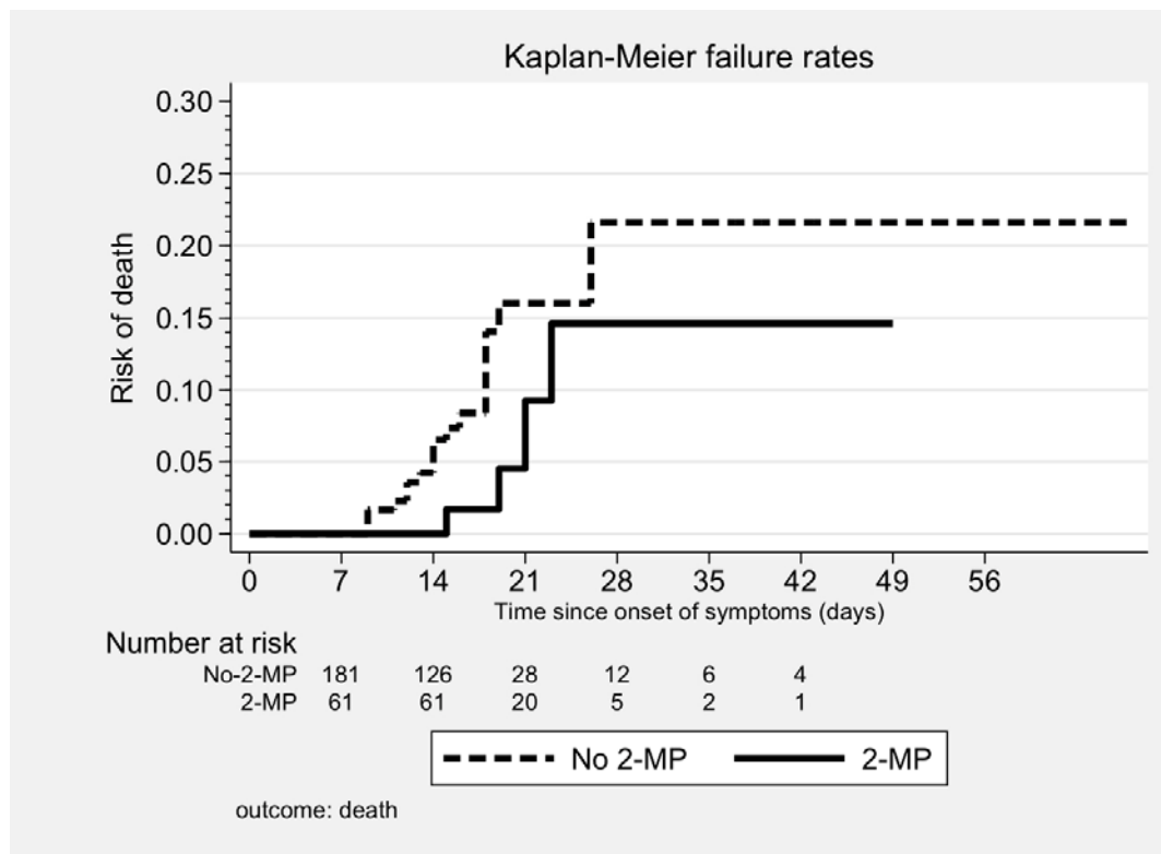
Figure 1. Kaplan-Meier failure curves. Outcome: death
