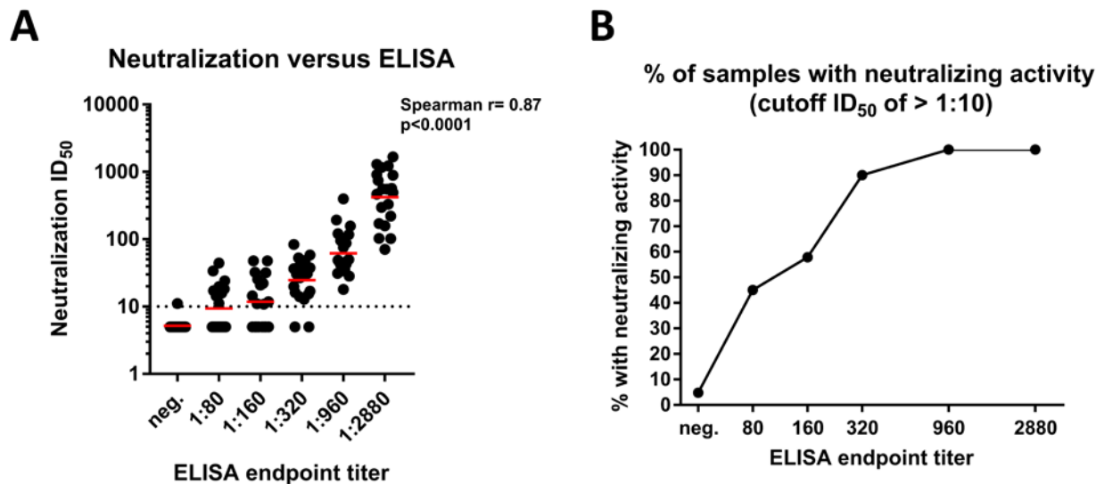
278 279 Figure 2. Neutralizing activity of serum samples in relation to ELISA titers. A shows a 280 correlation analysis between ELISA titers on the x-axis and neutralization titers in a 281 microneutralization assay on the y-axis. The Spearman r was determined. B shows the proportion 282 of sera that exert any neutralizing activity in each of the ELISA titer categories.
