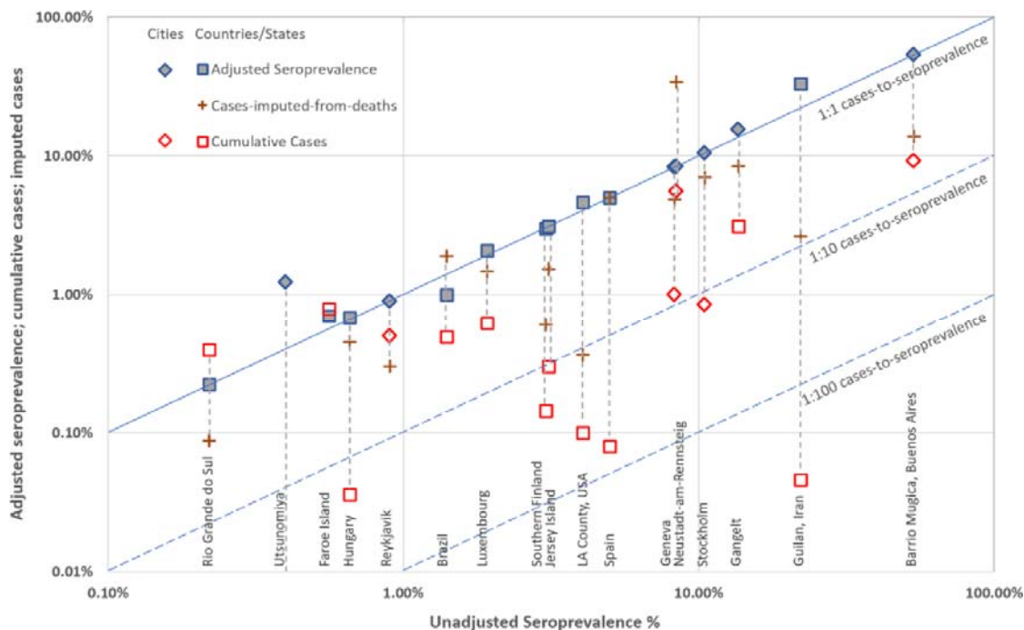
Figure 2. Log-log plot of study seroprevalence (x-axis) vs two cumulative case estimators for each study. Diagonal lines indicate rates equal to seroprevalence (solid) or 1/10 seroprevalence (dashed).
