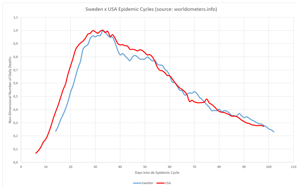
Figure 13 – Sweden and USA epidemic cycles compared, after their data being submitted to MAMI and non-dimension method.
