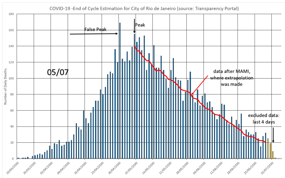
Figure 18 – Data extrapolation for end of cycle estimation using data collected in July the 5 th , 2020 The estimated end is at July the 07 th .
