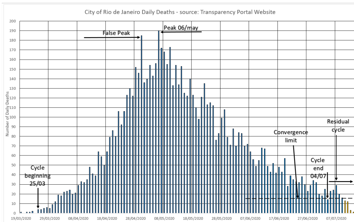
Figure 19 – The Rio de Janeiro’s cycle, closed already by the time this work was written, presented almost symmetrical ascent and descent times and number of deaths.
