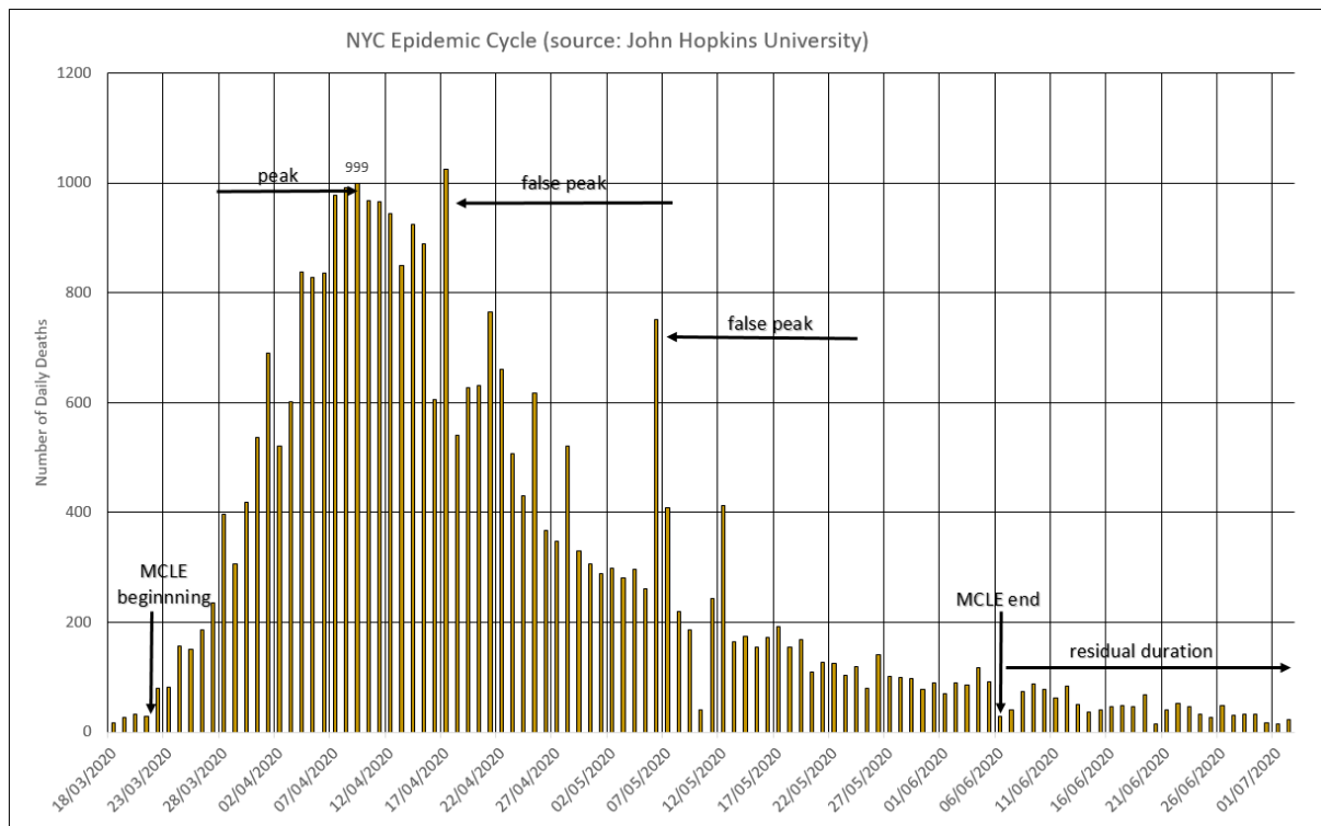
Figure 6 – New York’s MLCE
