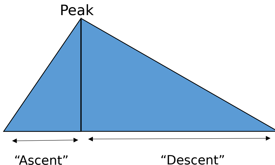
Figure 9 –COVID-19 lethal cycles generic shape.
