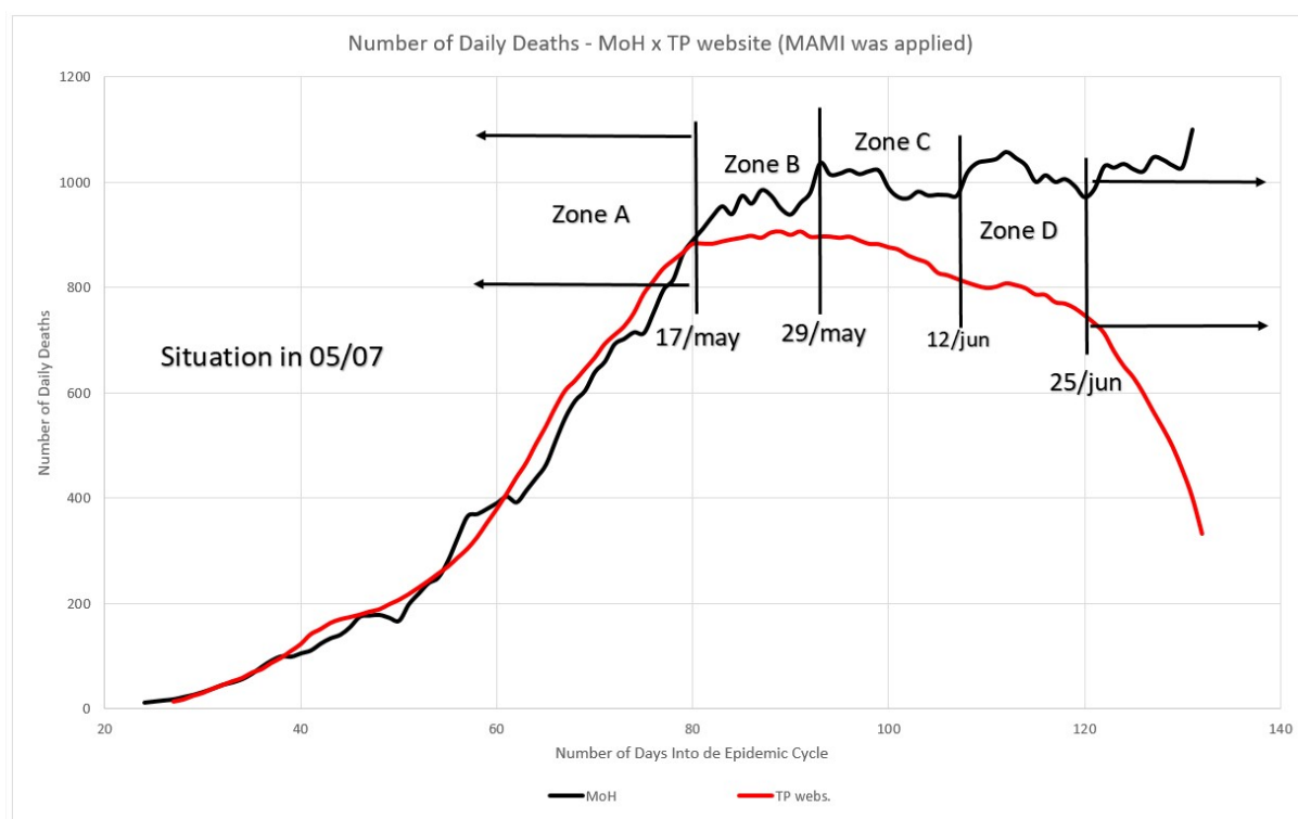
Figure A2 – Number of daily deaths according to MoH (black line) and Transparency Portal (red).
