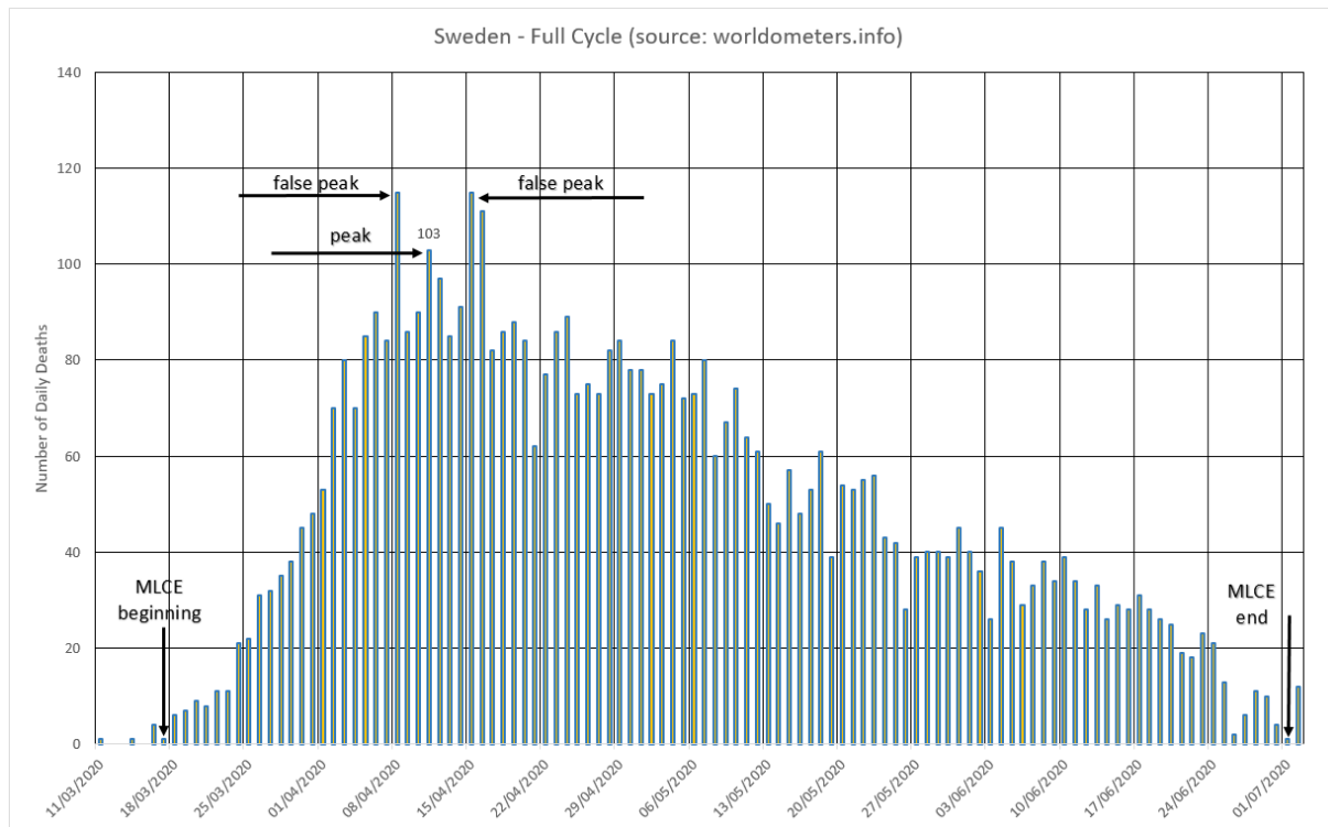
Figure 8 – Most Lethal Cycle of the Epidemic in Sweden.
