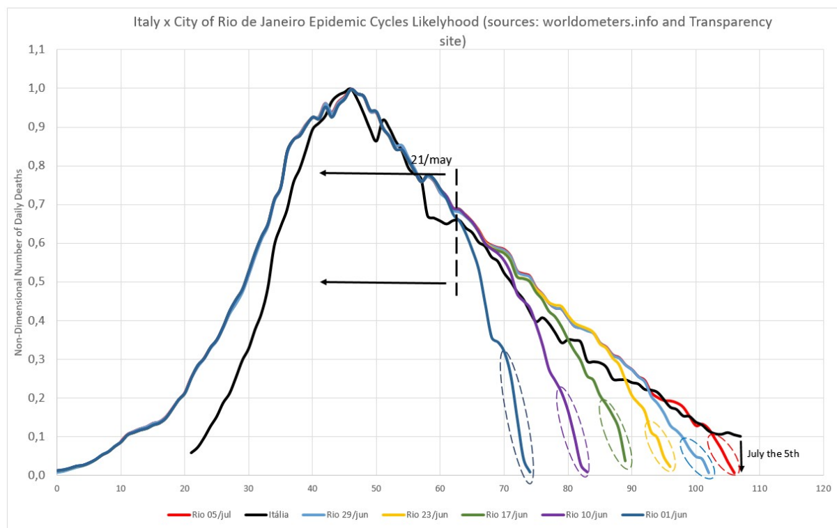
Figure 17 – Several evaluations for the end of the cycle comparing the city of Rio de Janeiro and Italy.
