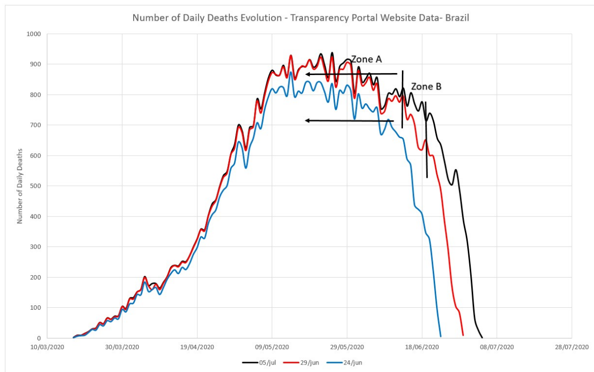
Figure 16 - Daily death figures data for Brazil, in three days. There are no noticeable difference between the second and the third weeks, only the last ten days.
