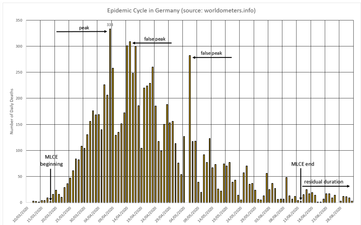
Figure 7 – The German cycle.
