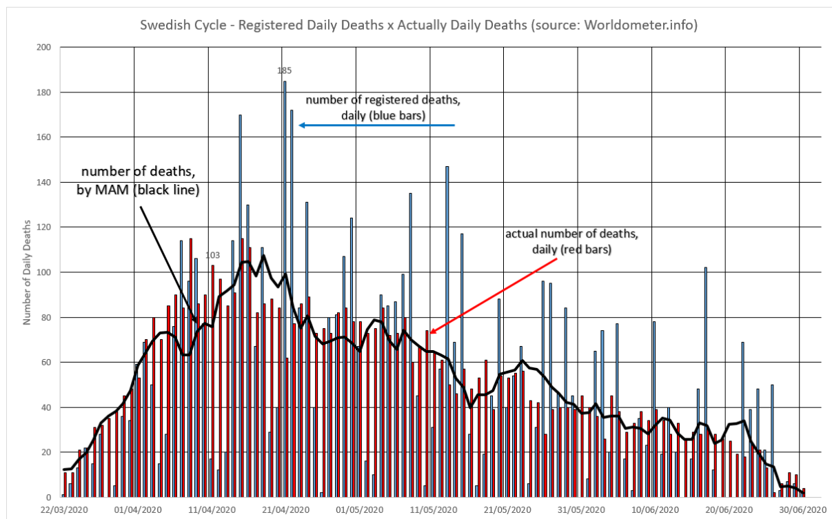
Figure 1 – Graphical match between data shown before for Sweden (number of registered deaths, daily – blue bars [6]) and the updated for actual number of daily deaths (red bars [7]). Black line represents the MAM figures.
