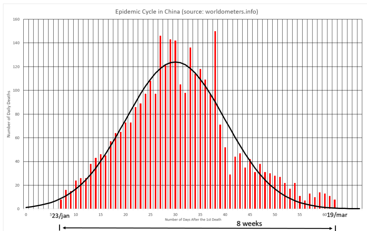
Figure 2 –COVID-19 deaths in China.
