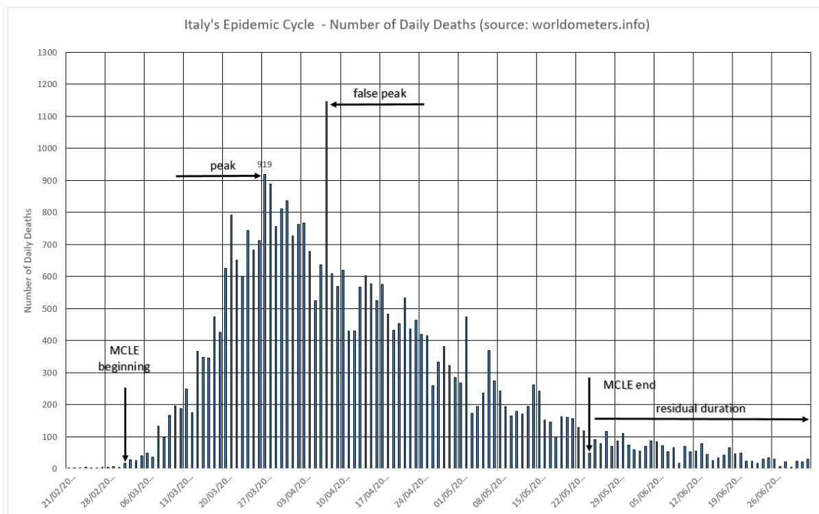
Figure 5 – The Italian cycle.
