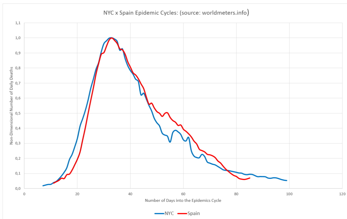
Figure 11 – NYC and Spain epidemic cycles compared, after their data being submitted to MAMI and non-dimension method.
