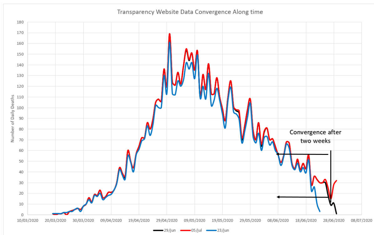
Figure 15 – Daily death figures data for City of Rio de Janeiro, in three days. There are no noticeable difference between the second and the third weeks, only the last four days.
