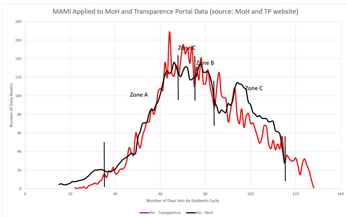
Figure A1 – MoH (black) x TP website (red) data comparison after MAMI.
