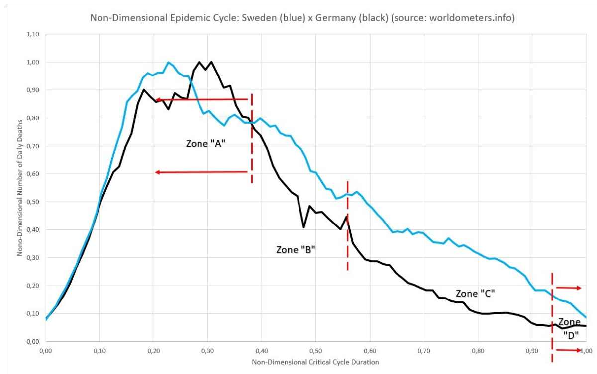
Figure 14 – Fully Normalized Sweden X Germany epidemic cycles compared.
