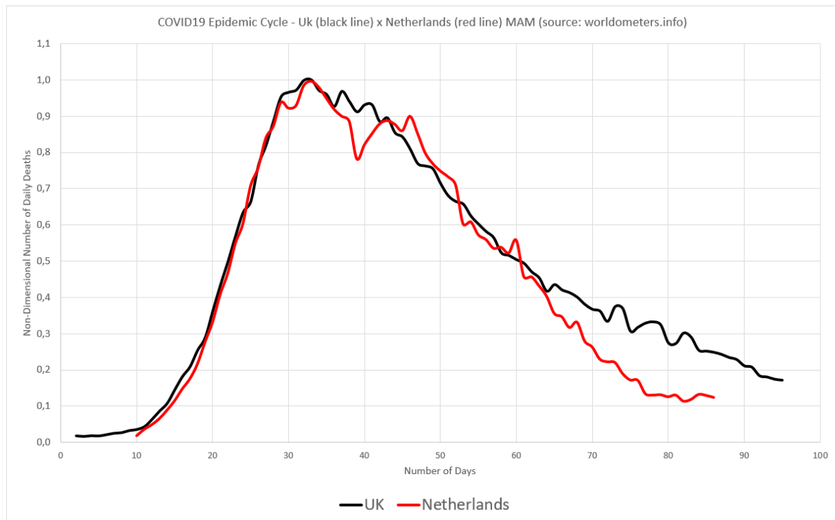
Figure 10 – UK and Netherlands epidemic cycles compared, after their data being submitted to MAMI and non-dimension method.
