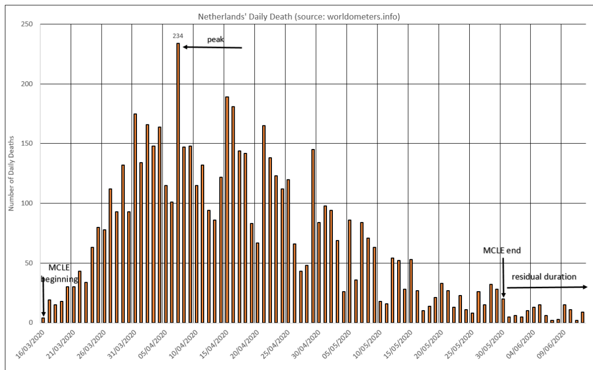
Figure 4 – Most Lethal Cycle of the Epidemic – The Netherlands (MLCE).
