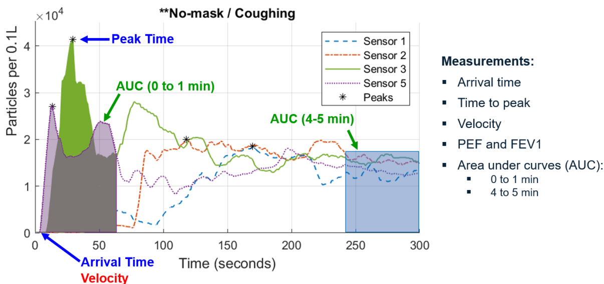
Figure 1: Examples of the measurements performed on the time-series data from all experiment runs for each of the four sensors and particle sizes of 0.3\mu\text{m} , 0.5\mu\text{m} , 1\mu\text{m} , 2.5\mu\text{m} , 5\mu\text{m} , 10\mu\text{m}
