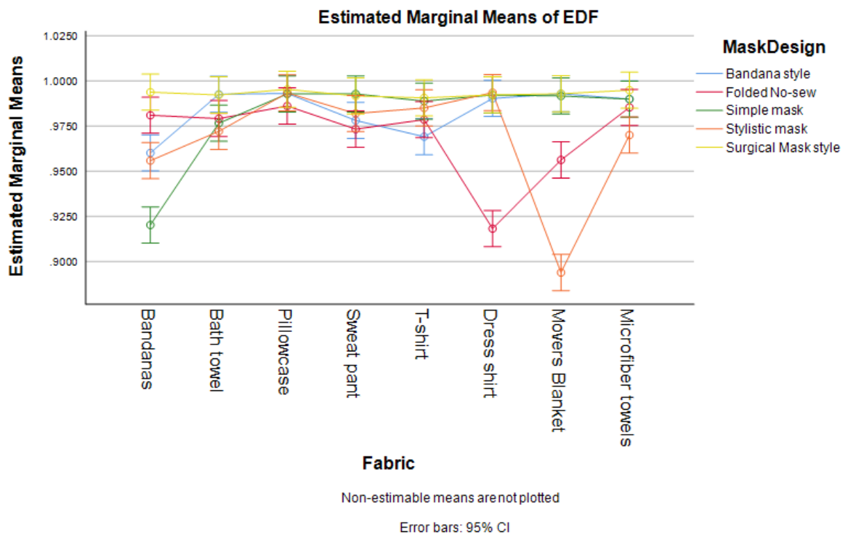
Figure 2: Estimated means of EDF resulting from MANOVA, showing the combined effects of fabrics and mask design. The test condition for “no-mask” resulted in particle cloud velocities that exceeded the sampling rate of the PMS sensors and were not captured. Consequently, an EDF for “no-mask” was not calculated.
