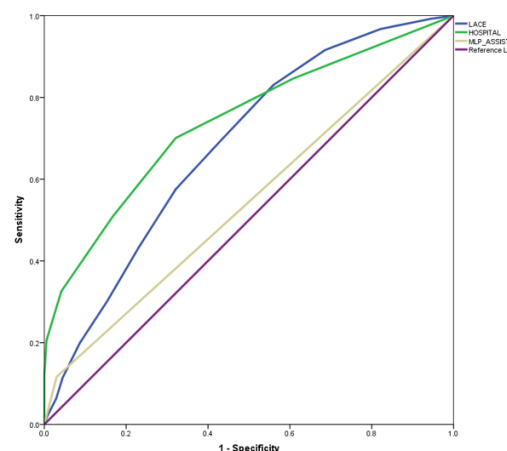
Figure 3. Receiver operating characteristic curves for the HOSPITAL score, LACE index, and the need for services from the MLP
