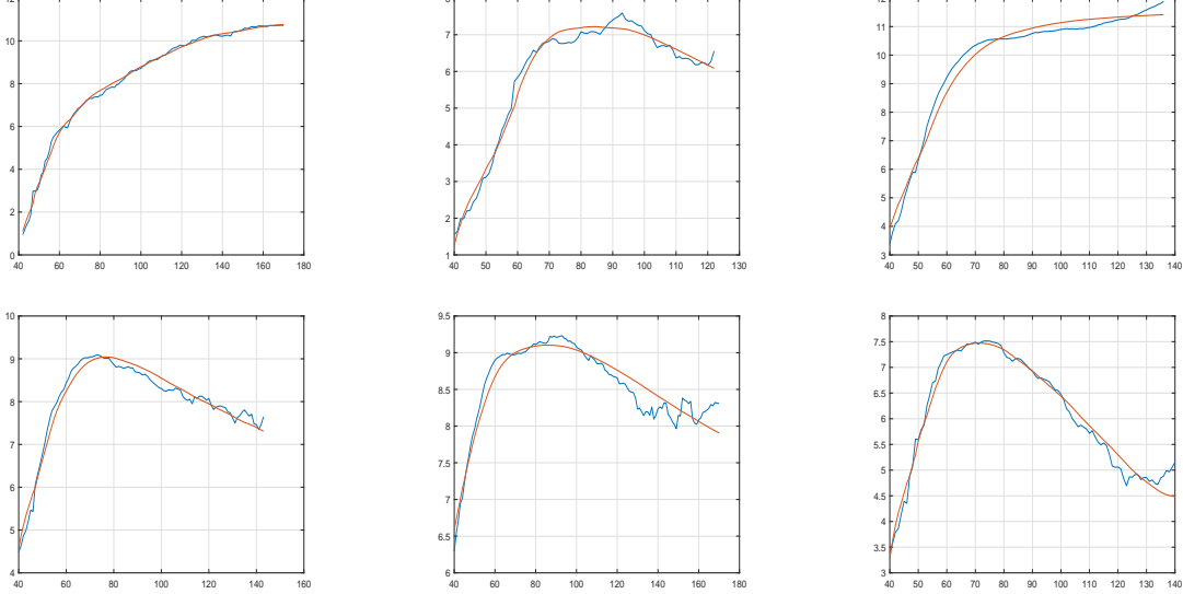
Figure 3: Logarithmic incremental affected cases (blue) and their linear regressions on logarithmic infected cases (red), each country in its training period. From top left to bottom right: Brazil, Israel, USA, Germany, Italy, Switzerland.
