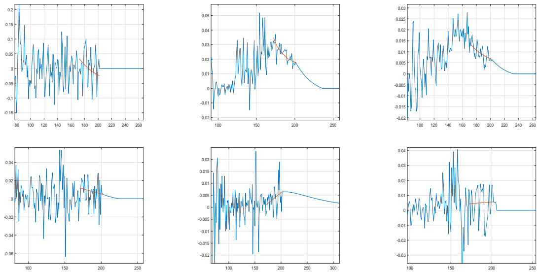
Figure 6: DLK: Incremental logarithmic ISPS. Empirical measurement until day 207 (August 15) and projected scenario beyond. From top left to bottom right: Brazil, Israel, USA, Germany, Italy, Switzerland.
