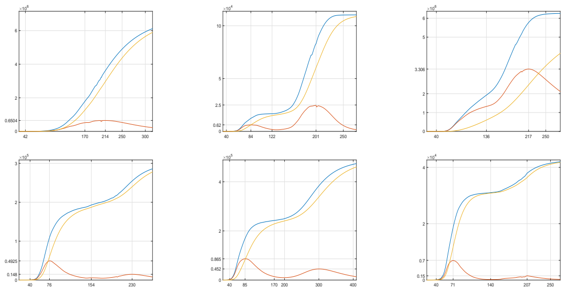
Figure 7: SIR equations solution under the scenario, with marked local maxima of the number of infected cases. From top left to bottom right: Brazil, Israel, USA, Germany, Italy, Switzerland.
