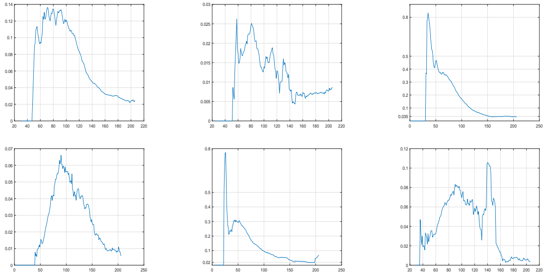
Figure 5: The proportion of incremental dead cases out of incremental removed cases. From top left to bottom right: Brazil, Israel, USA, Germany, Italy, Switzerland.
