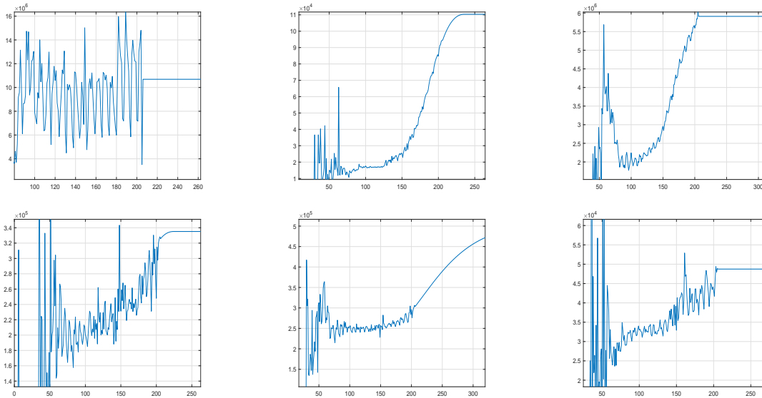
Figure 4: ISPS: Implied susceptible population size ISPS. Empirical measurement until day 207 (August 15) and projected scenario beyond. From top left to bottom right: Brazil, Israel, USA, Germany, Italy, Switzerland.
