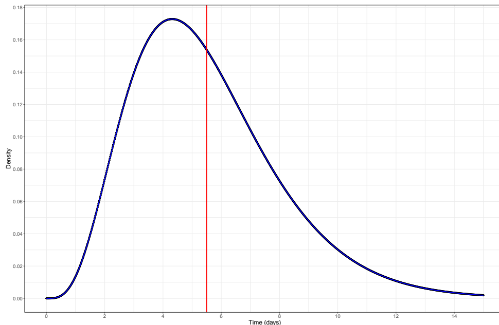
Figure 2: The communicable period: a = 4.7 , b = 0.85 . The mean of 5.5 days is indicated by the read vertical line.
