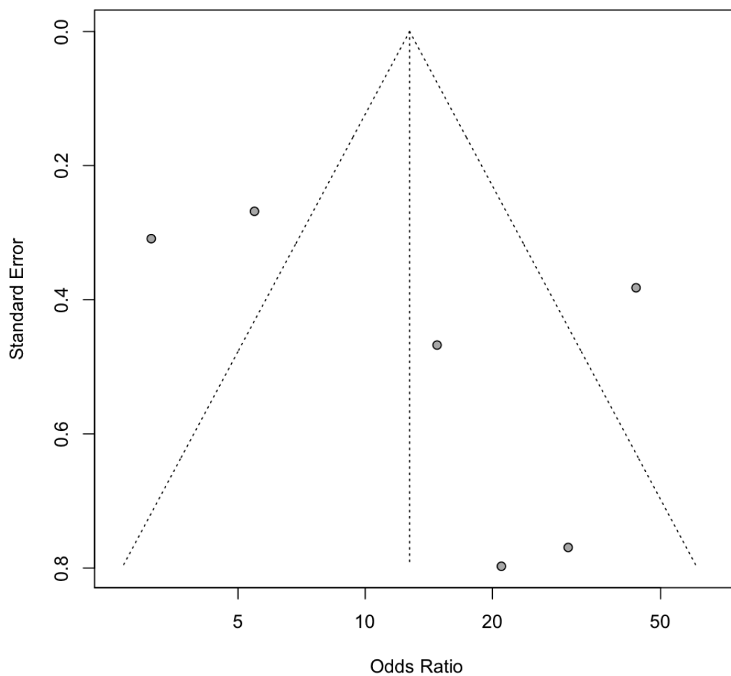
Figure 5: Publication bias by Begg's funnel plot for overall pooled diagnostic effect
