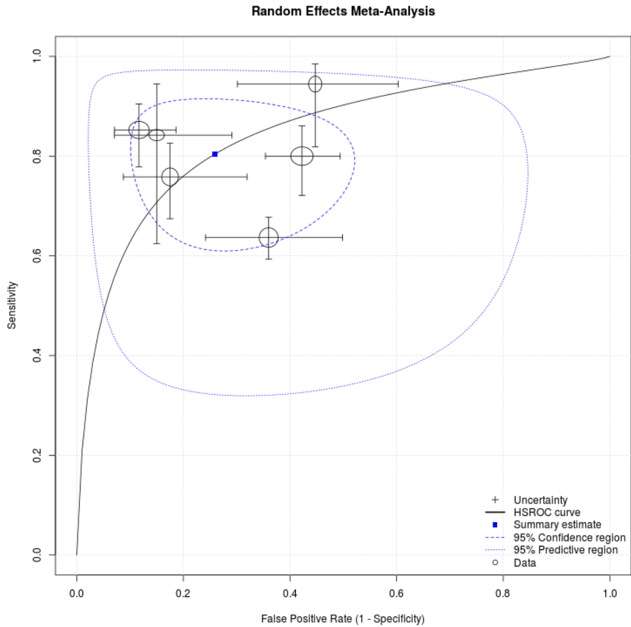
Figure 4: ROC plot displaying extrapolated SROC curve, the summary estimate for sensitivity and specificity, and percentage study weights
