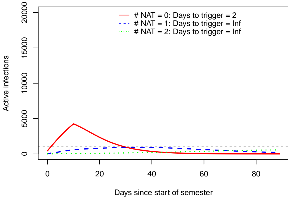
R0 = 1.25
