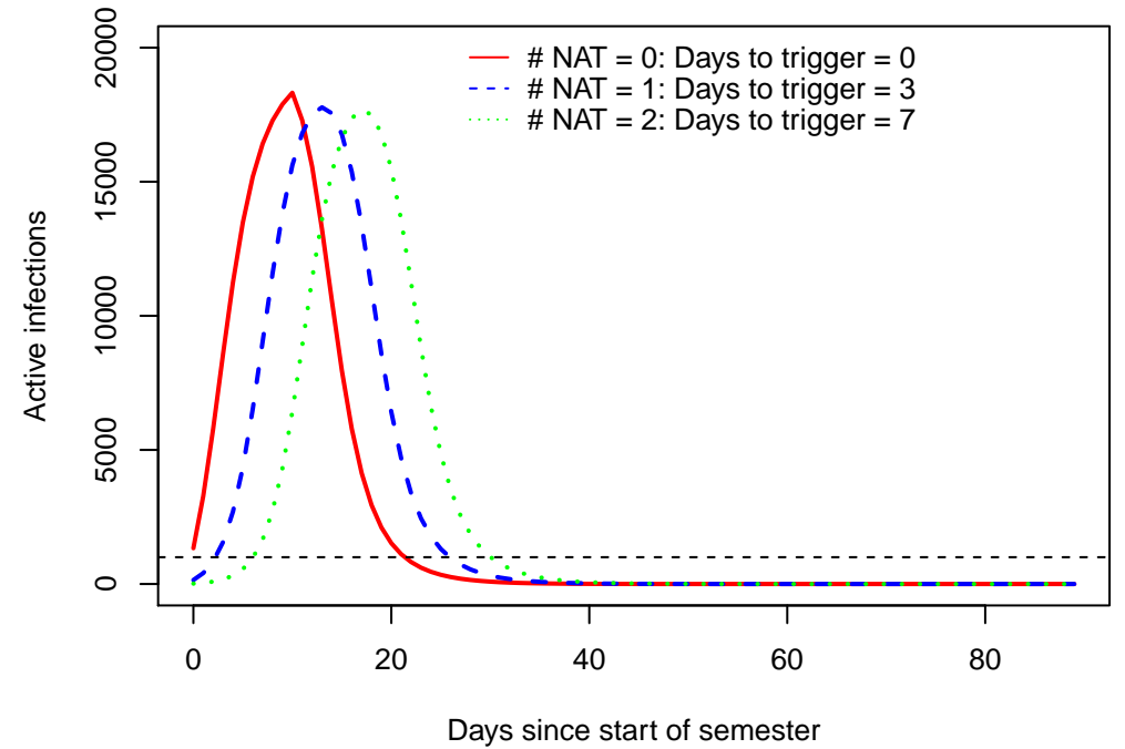
R0 = 3
