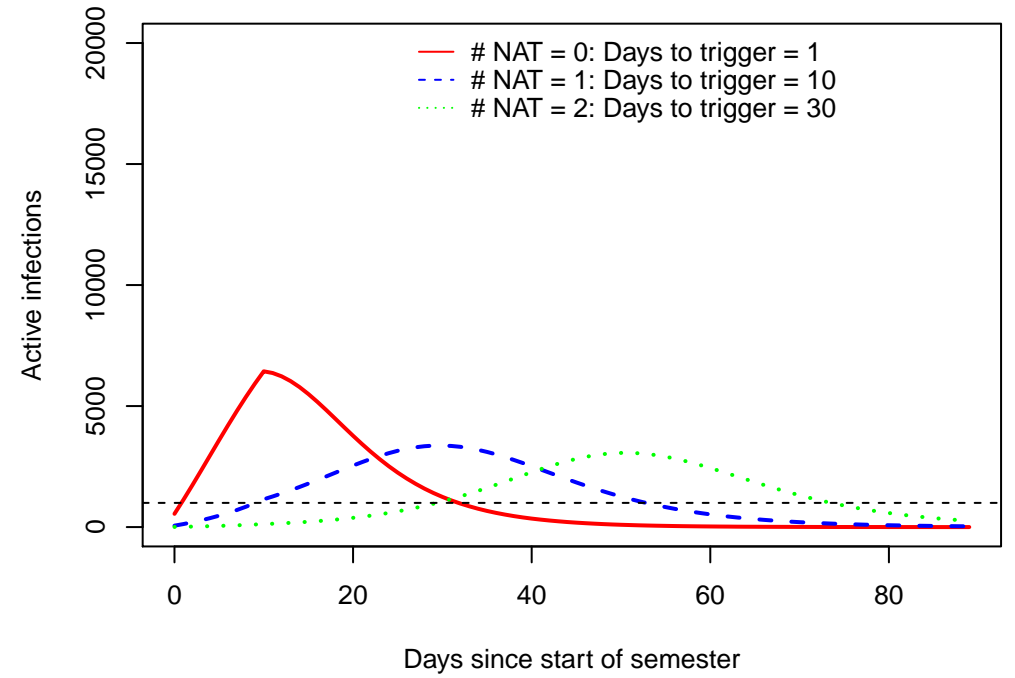
R0 = 1.5
