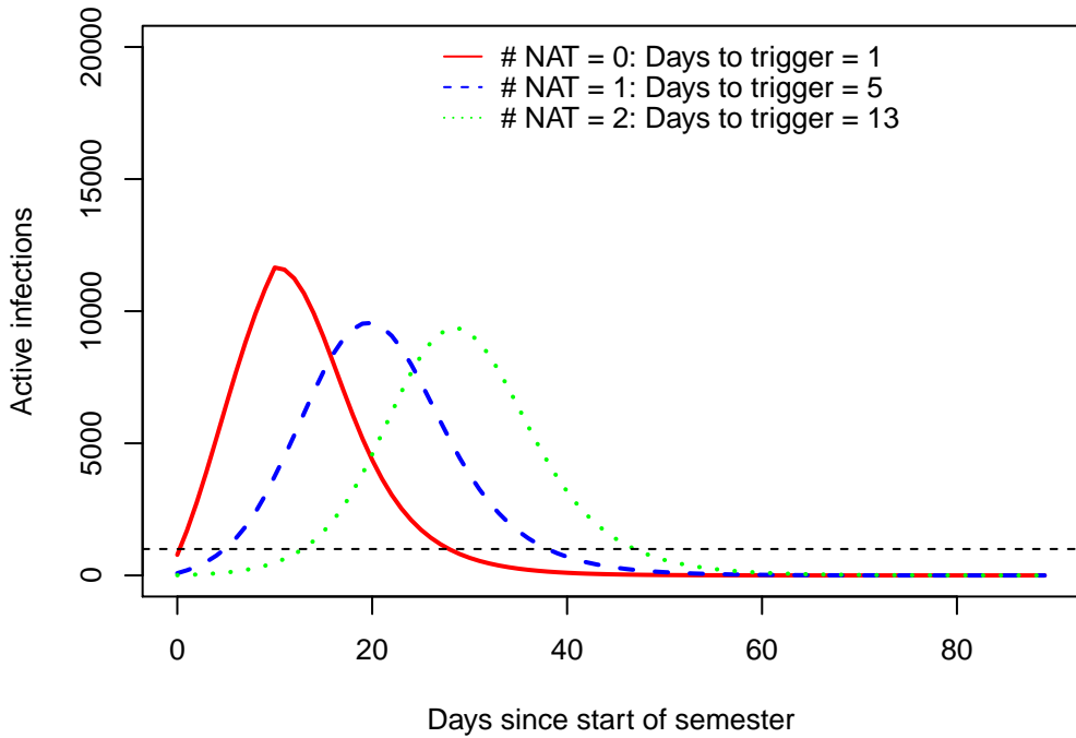
R0 = 2
