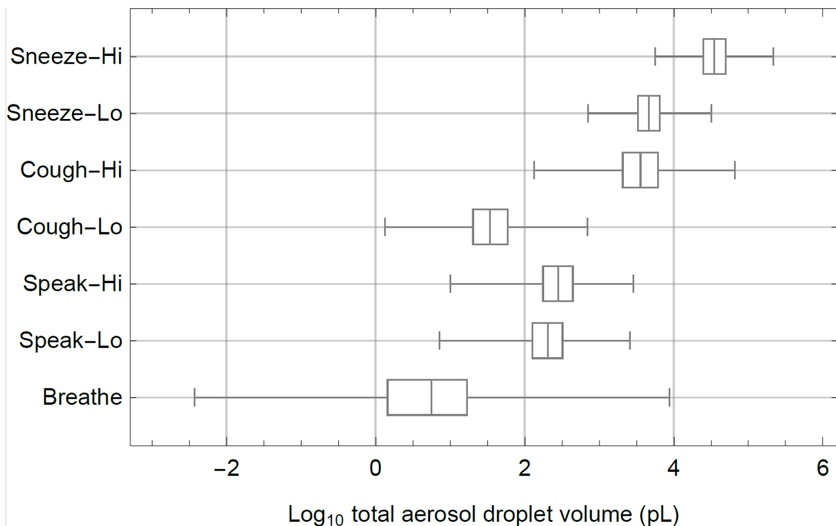
675 Figure 2. Box-whisker chart of the \log_{10} of total aerosol droplet volumes (pL=picolitres) that are 676 expelled in each scenario (Table 1), showing median values, quartiles (boxes) en minimum and 677 maximum values (whiskers). Volumes in pL/20 minutes for breathing and speaking and in pL per 678 cough and per sneeze.
