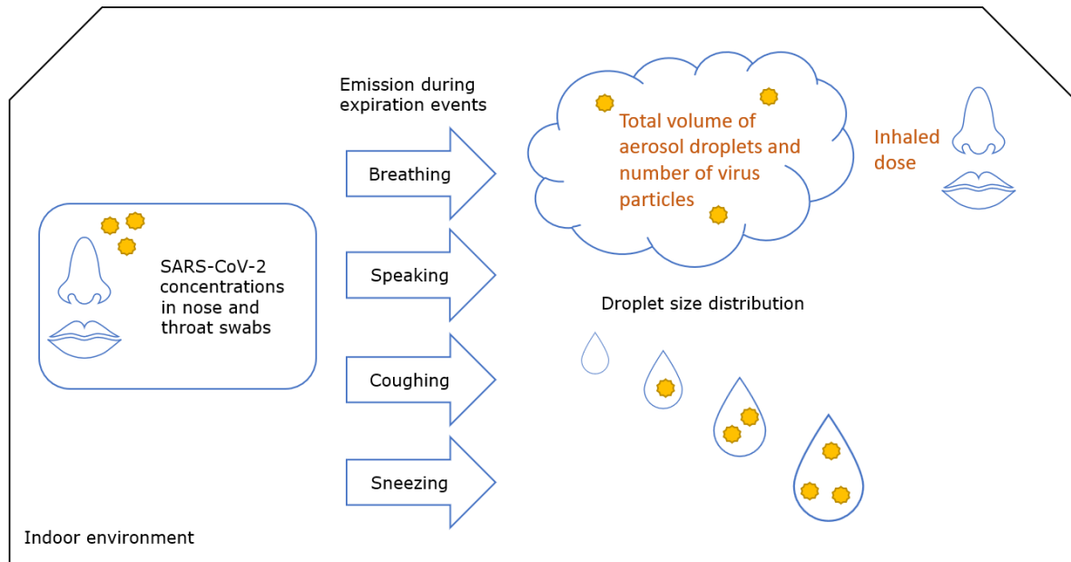
672 Figure 1. Overview of the processes modelled in this study.
