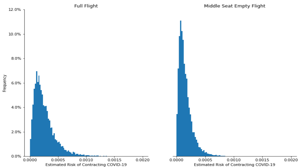
Distribution of Estimated Risk of Contracting Covid-19 on a US Domestic Jet Flight Two Hours Long, Based on 10,000 Simulations
