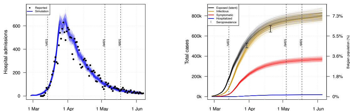
Figure S7: Daily hospital admissions (left) and cumulative number of exposed, infectious and symptomatic cases(right) over time with age-specific susceptibility The cumulative numbers are presented together with confidence intervals from serial seroprevalence data on 30th March and 20th April based on [19].
