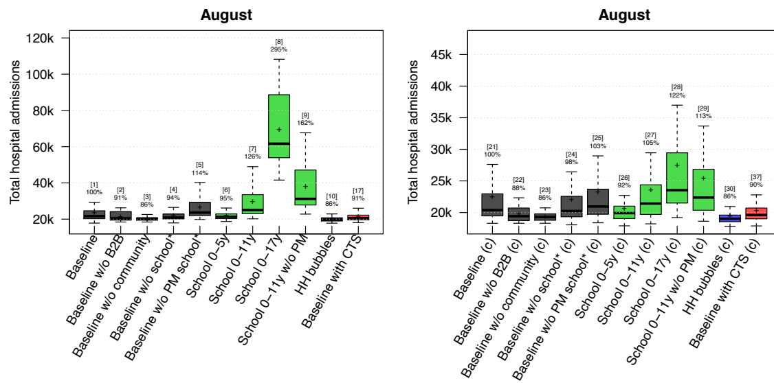
Figure 4: Predicted cumulative hospital cases on 31 August assuming that children (0-17y) are equally susceptible as adults (left) or only half as susceptible compared to adults (right). The results are presented as the median, the 75% (box) and 95% (whiskers) percentile and average (cross) for all combinations of the contact reductions per scenario. The numbers on top of the whiskers indicate the scenario number from Table 1 and the relative change in the scenario average with respect to the baseline. HH: Household, w/o: without, CTS: contact tracing strategy; PM: precautionary measures at school.
