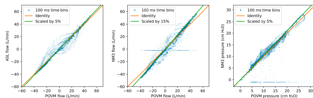
Fig 14. Fine comparison of Princeton Open Ventilation Monitor (POVM), the artificial lung simulator (ASL), and a commercial respiratory monitor (NM3) in matched time-bins (100 ms wide). The commercial monitor occasionally drops to zero and has discretization effects at low pressure. POVM and ASL agree in flow up to a 5% scale factor; POVM and NM3 agree in flow up to a 15% scale factor, and POVM and NM3 agree in pressure up to a 5% scale factor.
