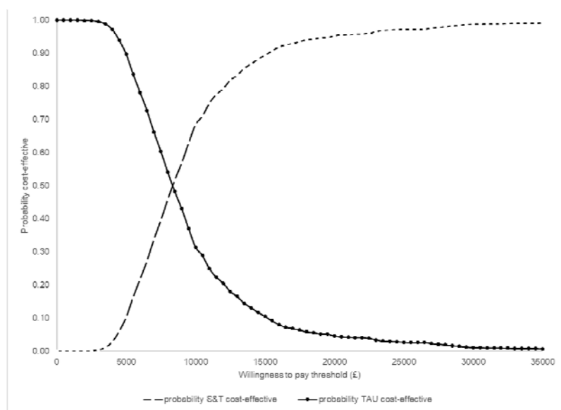
Figure 3: Cost-effectiveness acceptability curve
