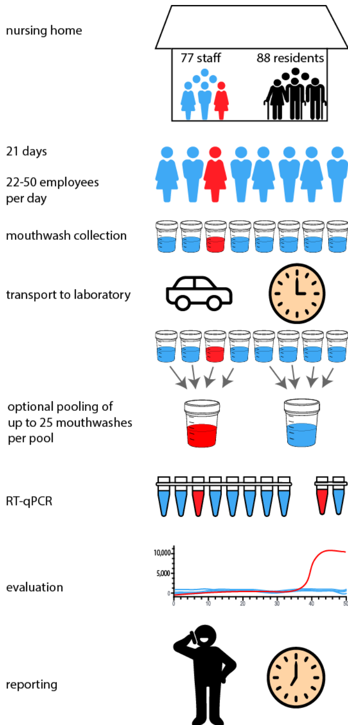
Figure 4. Daily testing of personnel of a nursing home with or without pooling of mouthwashes. Red color indicate a SARS-CoV-2 positive individual/sample.
