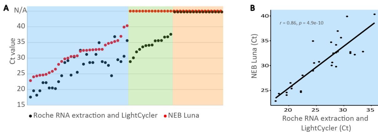
Figure 3. (A) Roche RNA extraction/RT-qPCR and NEB Luna RT-qPCR for SARS-CoV-2 detection in 62 mouthwash samples from hospital patients. The NEB method detects the virus
