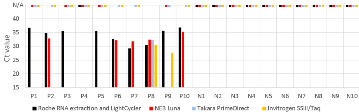
Figure 1. RT-qPCR of 10 previously SARS-CoV-2 positive (P) and 10 previously SARS-CoV-2 negative (N) mouthwashes. RNA was either extracted from 200 \mu l of mouthwashes (black bars) or 1 \mu l of the mouthwashes was added directly to the RT-qPCR reaction mix without prior extraction (colored bars). Dashes at N/A indicate no amplification of the viral target.
