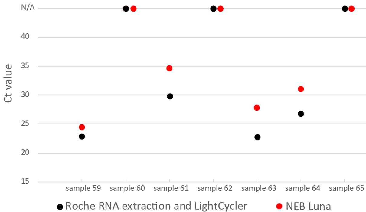
Figure 2. Roche RNA extraction/RT-qPCR and NEB Luna RT-qPCR of seven reference samples. Dots at N/A show no amplification of the viral target.
