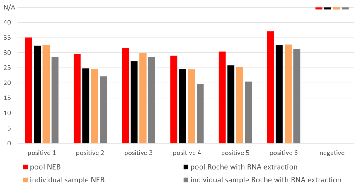
Figure 5. Tests of seven pools of 26 mouthwash samples, which in six cases contain one positive sample. Dashes at N/A show no amplification of the viral target.
