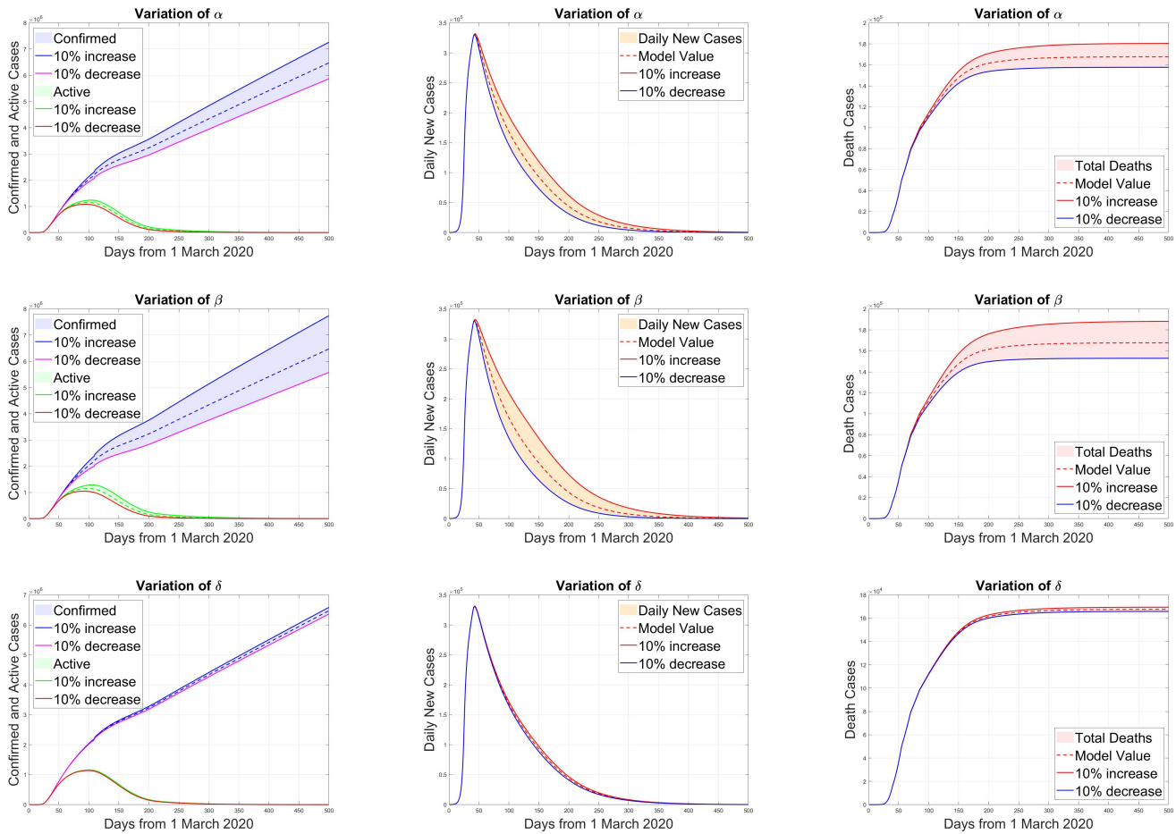
Fig. 12: Sensitivity Study for the rate of transmission of infection \alpha, \beta and \delta . The Variation in total confirmed cases, total active cases and Extinct cases is plotted for 10% increase and decrease in the parameter value from the optimized value.
