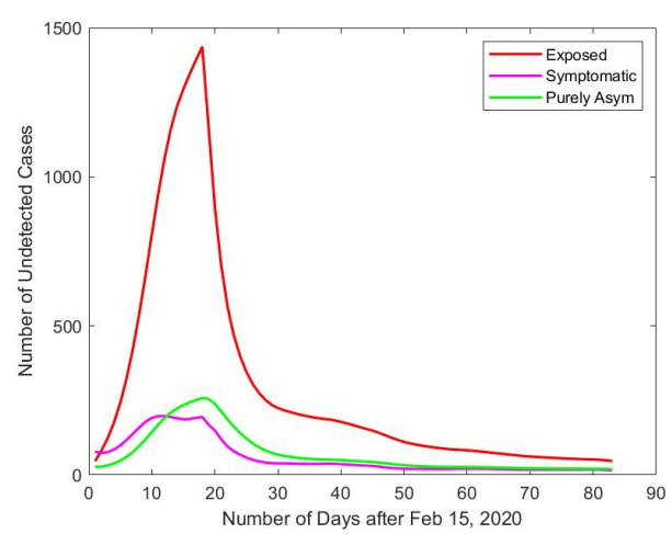
d. Undetected Exposed, Symptomatic and Asymptomatic Cases
