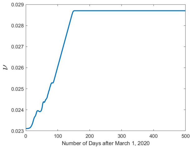
c. Detection rate of Symptomatic cases for USA
