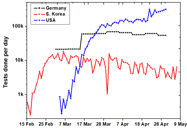
a. Daily Tests per day for South Korea, Germany and USA
