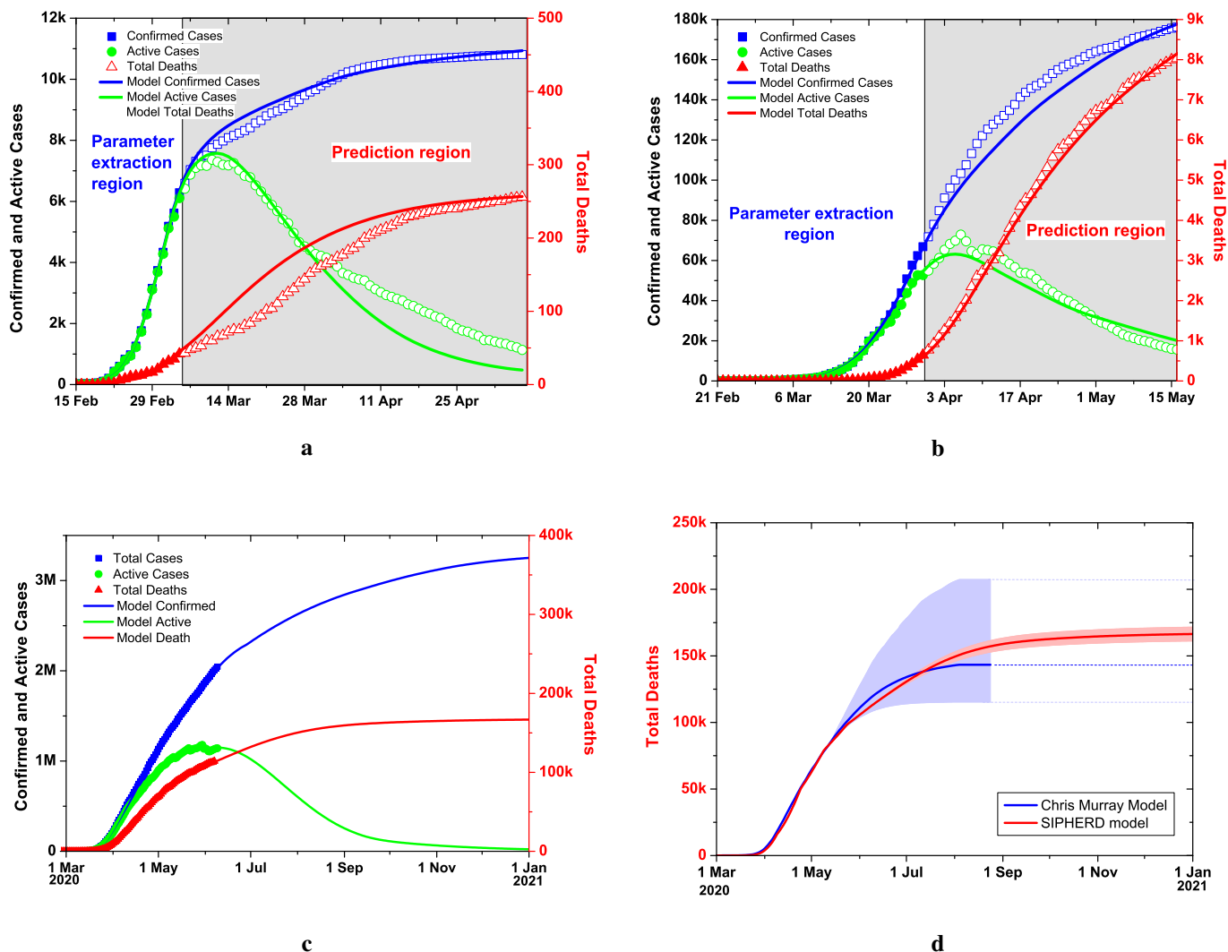
Fig. 2: Model predictions for South Korea, Germany and USA. a. South Korea data given to the simulator up-to March 5, and thereafter, model comparison with the actual data for the confirmed, active cases and total deaths. b. Model prediction using the Germany data up-to March 31 and comparison with the actual data for the confirmed, active cases and total deaths. c. Comparison of the Model prediction for USA if the social distancing and lockdown conditions kept same and relaxed after June 15 while the tests increased by 10k daily for both scenarios. d. SIPHERD Model compared with 'Cris Murray Model' for the projection of the extinct cases.
