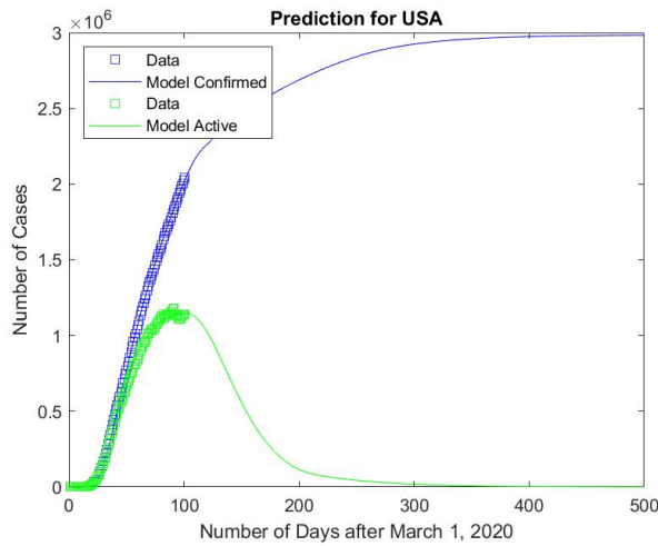
a. Confirmed and Active cases data Vs Model Prediction
