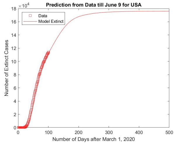
c. Total Extinct Cases
