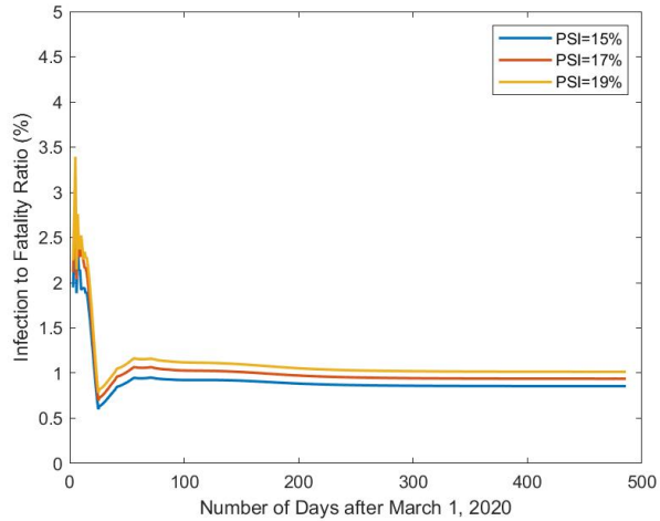
c. Infection to Fatality Ratio (%) for different P_{SI} values.
