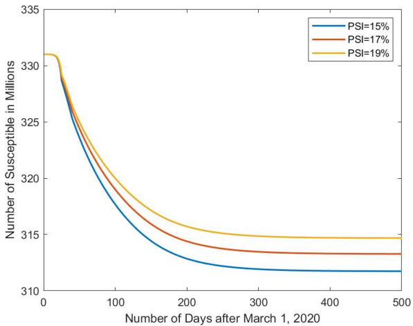
a. Number of Susceptible people for different P_{SI} values.
