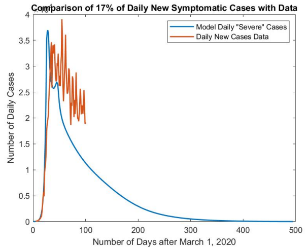
d. Daily new cases data compared with Daily Symptomatic Severe cases for 17% P_{SI} .
