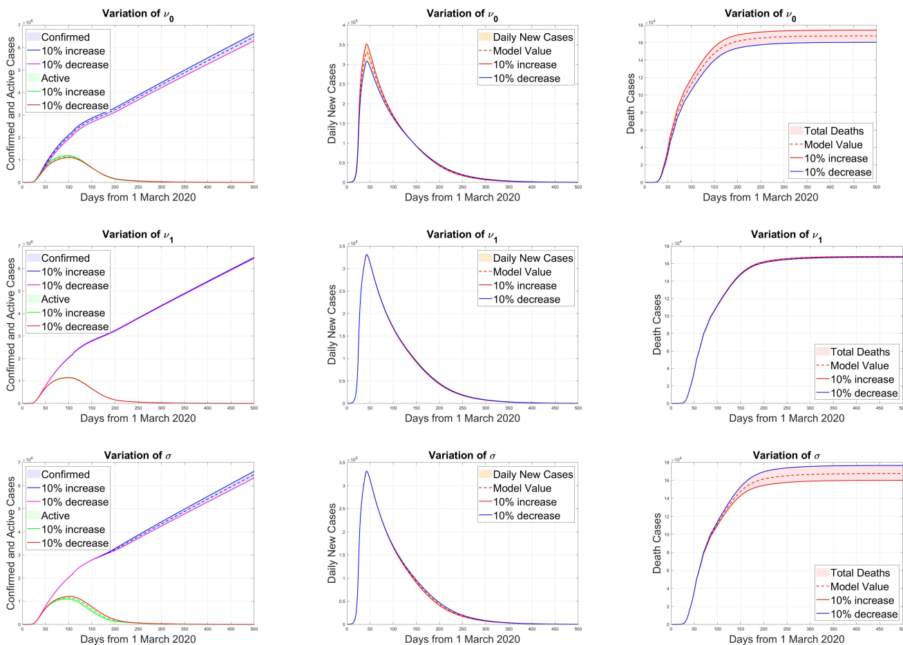
Fig. 11: Sensitivity Study for the detection rate constants \nu_0, \nu_1 and recovery rate \sigma . The Variation in total confirmed cases, total active cases and Extinct cases is plotted for 10% increase and decrease in the parameter value from the optimized value.
