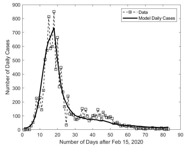
b. Daily new cases data compared with Model Prediction
