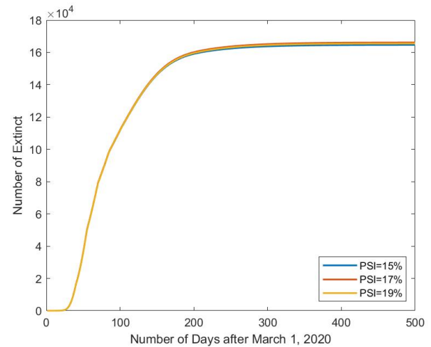
b. Total Extinct cases for different P_{SI} values.
