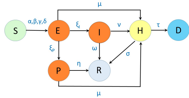
Fig. 1: Schematic of the SIPHERD Model: \alpha, \beta, \gamma, \delta are rates of transmission of infection; \xi_I, \xi_P are rates of transfer from exposed to Symptomatic and Asymptomatic; \omega, \eta, \sigma are recovery rates; \mu, \nu are detection rates, and \tau is mortality rate.
