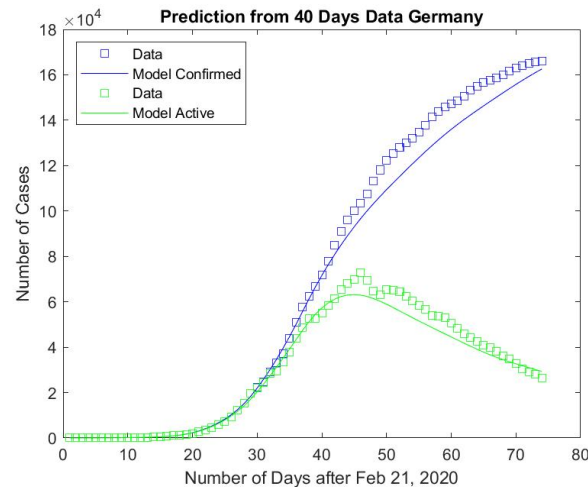
a. Total Confirmed and Active cases data Vs Model Prediction
