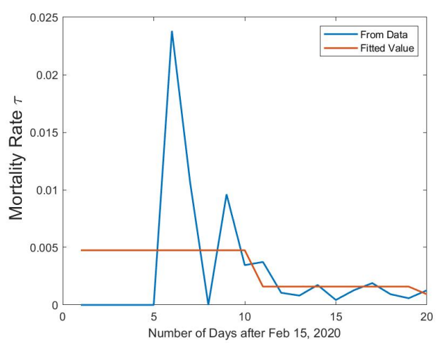
f. Mortality rate from the data and the fit
