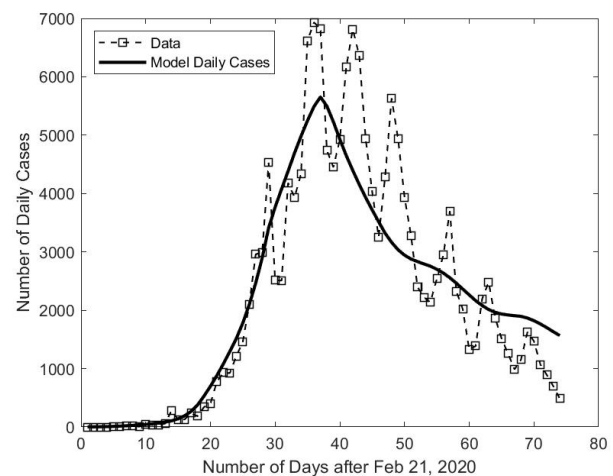
b. Daily new cases data compared with Model Prediction
