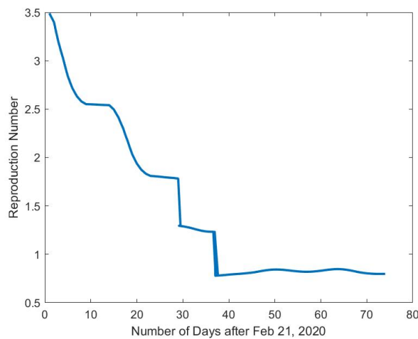
e. Basic Reproduction Number
