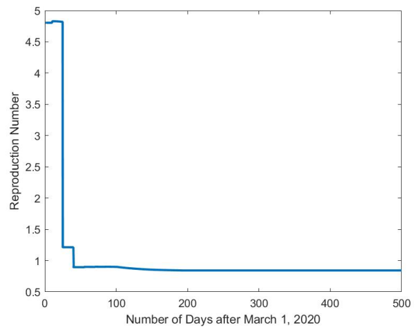
f. Basic Reproduction Number
