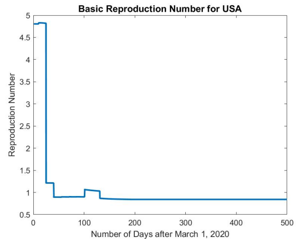
f. Basic Reproduction Number
