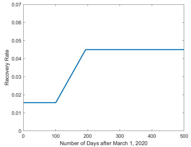
d. Recovery rate from optimizer and linear fit for USA
