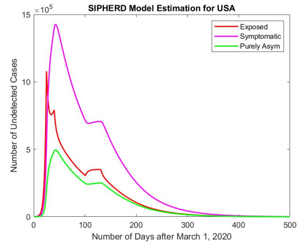
d. Undetected Exposed, Symptomatic and Asymptomatic Cases
