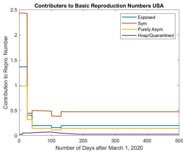
e. Different Infection category contribution to the Basic Reproduction Number
