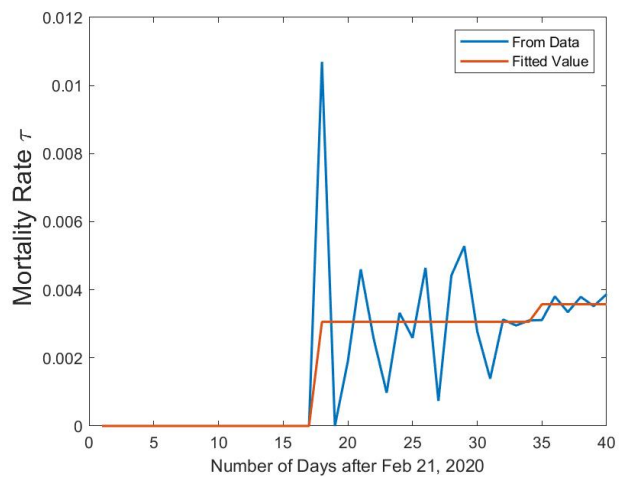
f. Mortality rate from the data and fit
