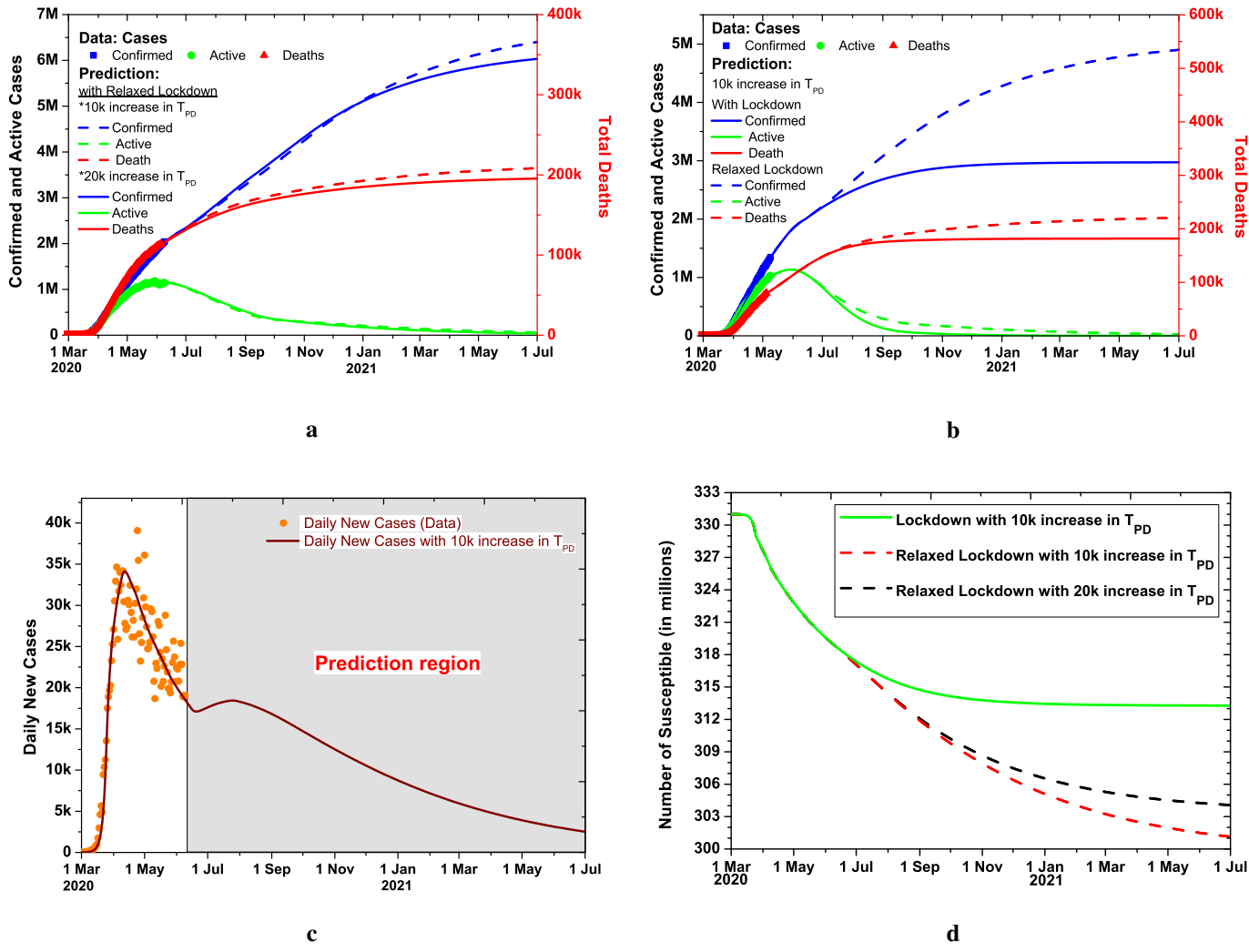
Fig. 4: Effect of increased tests and relaxed lockdown. a. Effect of increased testing on the total, active and extinct cases, comparison of 10k and 20k increase in Tests per day ( T_{PD} ) saturated at 1 million and 2 million respectively b. Comparison of the Total, Active and extinct cases in lockdown and relaxed lockdown situation c. Model prediction for daily new cases with the increase of 10k tests per day with lockdown conditions relaxed after June 15 d. The evolution of the Susceptible when lockdown situations kept same and relaxed after June 15 with tests per day increase by 10k and 20k.
