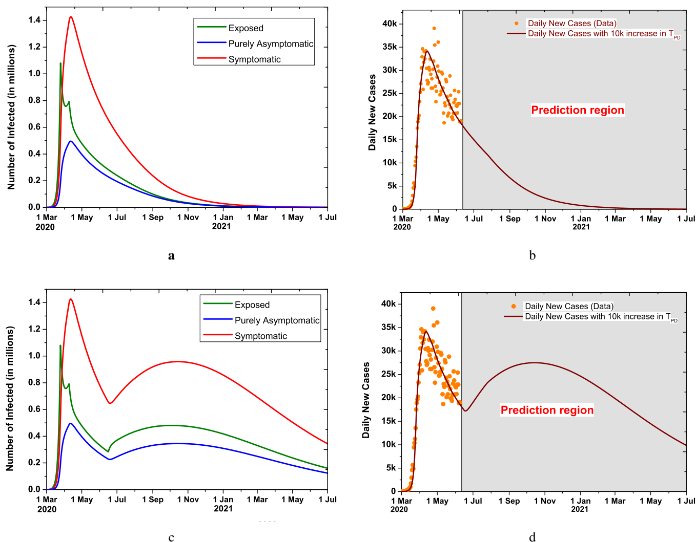
Fig. 3: Possibility of a Second Wave of Infection. a. The evolution of the undetected number of Infected in Exposed (E), Symptomatic (I), and purely Asymptomatic (P) category with lockdown conditions kept the same. b. Model prediction for daily new cases for USA with the increase of 10k tests per day with lockdown conditions kept the same. c, d. The evolution of the undetected number of Infected in Exposed (E), Symptomatic (I) and purely Asymptomatic (P) category and Daily new cases when lockdown situations relaxed after June 15 to the extent that rate of transmission of infection increases by 30%.
