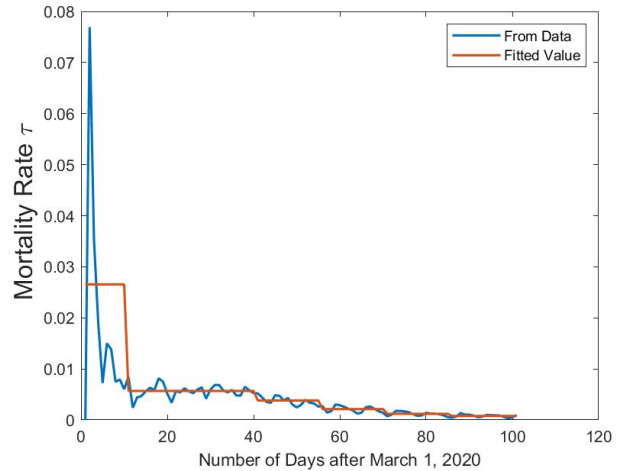
b. Mortality rate from the data and fit for USA
