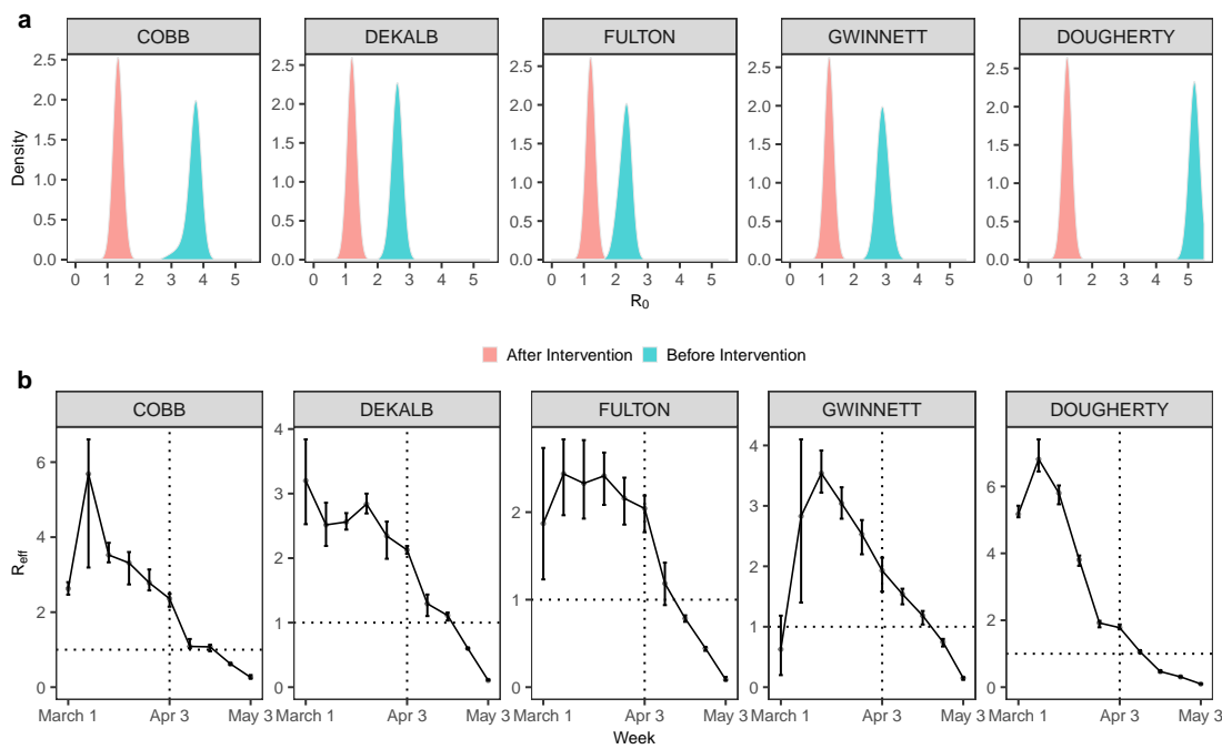
Fig. 1. Posterior distribution of basic reproductive number R_0 and the effective reproductive number R_{eff} , before and after the implementation of state-wide shelter-in-place order on April 3, 2020. Errorbars represent 95% credible interval.
