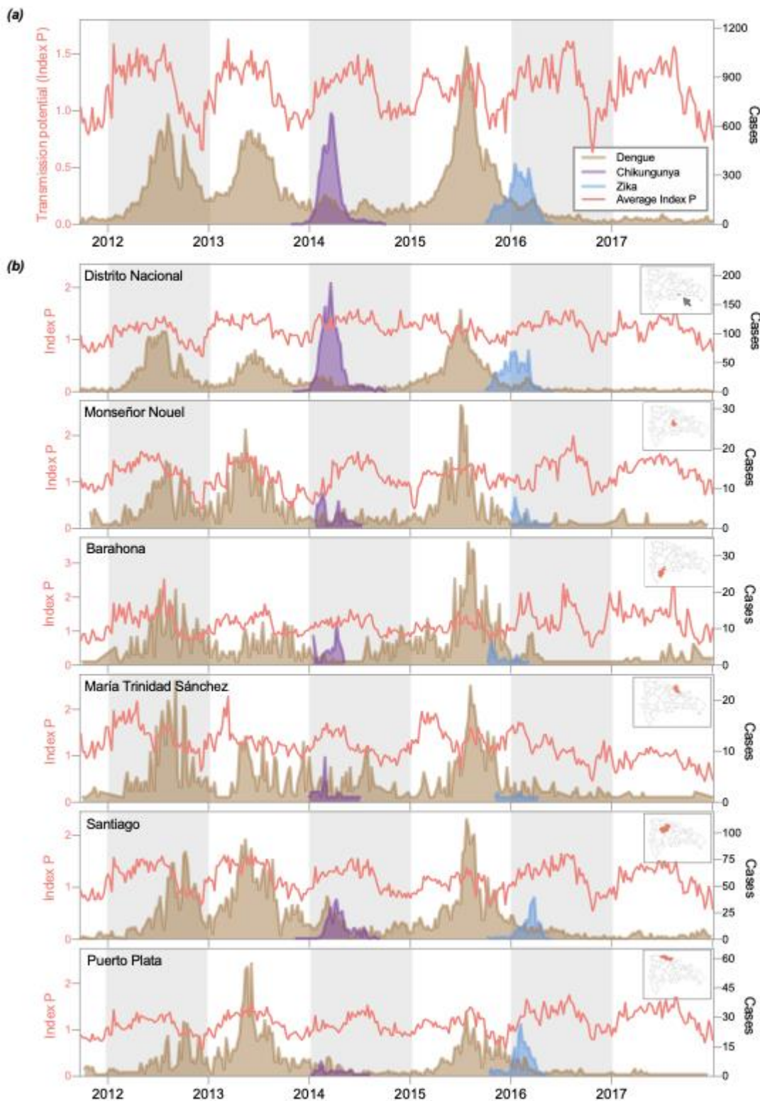
Figure 2. Emerging disease outbreaks occurred during periods of sub-optimal climate. (a) Average weekly transmission potential ( Index P ) and nationally reported cases. Index P describes the reproductive potential of an individual female Aedes mosquito, meaning its absolute value should be interpreted biologically rather than epidemiologically. Relative fluctuations in Index P reflect seasonal changes in the expected rate of mosquito-borne virus transmission. (b) Index P and reported cases for six provinces. Temperature and humidity data were retrieved from the National Meteorology Office (ONAMET) database (saip.gob.do) for Distrito Nacional, Barahona, Puerto Plata, María Trinidad Sánchez, and Santiago. Hourly climatological data for Monseñor Nouel
