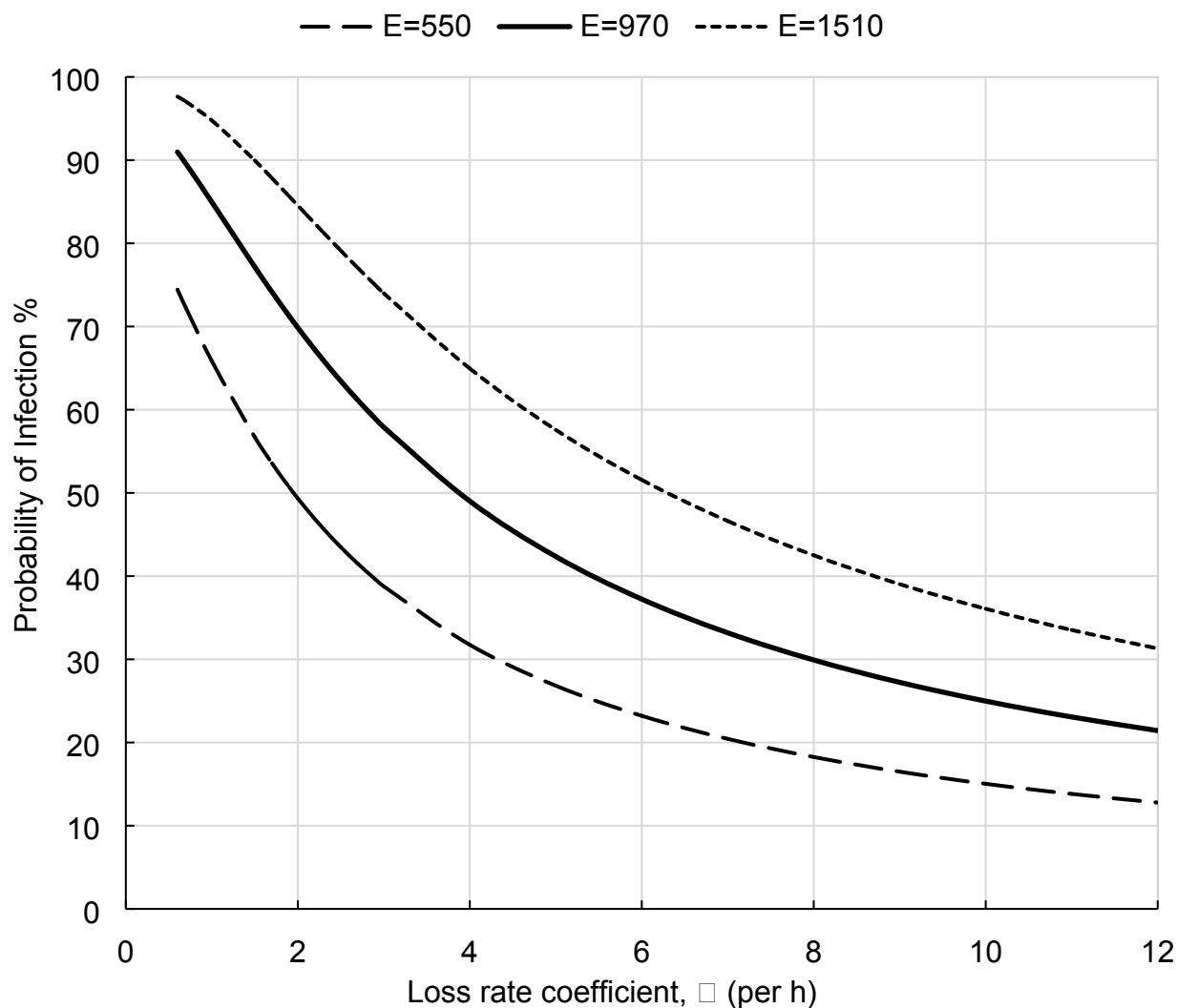
Figure 1. Probability of infection for each rehearsal participant as a function of loss rates for varying airborne quanta emission rates ( E , q\ h^{-1} ). Infection probability is plotted for the predicted mean emission rate ( 970\ q\ h^{-1} ) and the 10 th and 90 th percentile emission rates ( 550 and 1510\ q\ h^{-1} , respectively.) A rehearsal duration of 2.5 hours, an indoor volume of 810\ m^3 and a volumetric breathing rate of 1.0\ m^3\ h^{-1} were assumed.
