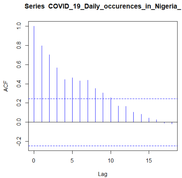
Fig 4: ACF Plot
