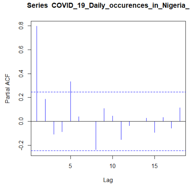
Fig 5: PACF Plot
