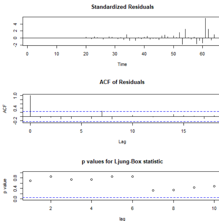
Fig 6: Diagnostic plot
