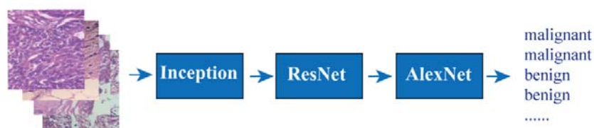
Figure 1. the architecture of DeepBC
