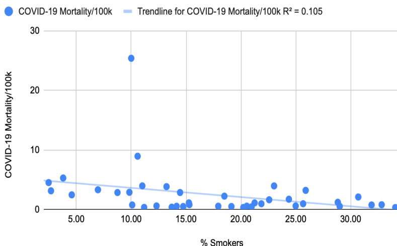
Figure 3. Daily smoking prevalence correlated inversely with national COVID-19 mortality rates for the combined group of the 20 hottest countries and the 20 coldest countries. Pearson's correlation without adjustments: R = -.324 , p = .0207 .
