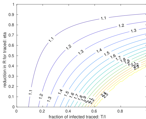
FIGURE 1. \mathcal{R}^{LD} needed to keep the observed reproduction number \mathcal{R} = 1 for various choices of tracing parameters T/I and \eta . Plot assumes \mathcal{R}_0 = 2.5 and s = 1 .
