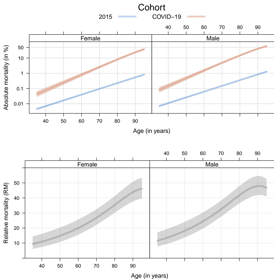
Supplementary Figure 8: Swiss 2015 population and covid-19 cohorts. Comparison of absolute mortality (the probability of dying from any cause after 60 days, plotted on logarithmic scale) between the Swiss 2015 population and covid-19 cohorts, separately for females and males of different ages (top). Comparison of relative mortality (RM, the ratio of absolute mortalities in the covid-19 versus the 2015 cohort) between the two cohorts, for females and male of different ages (bottom). All estimates are plotted with 95% confidence bands.
