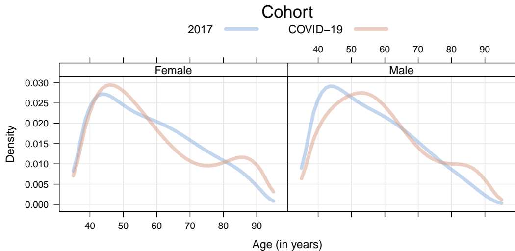
Supplementary Figure 3: Swiss 2017 population and covid-19 cohorts. Comparison of age densities between the Swiss 2017 population and covid-19 cohorts, separately for females and males.
