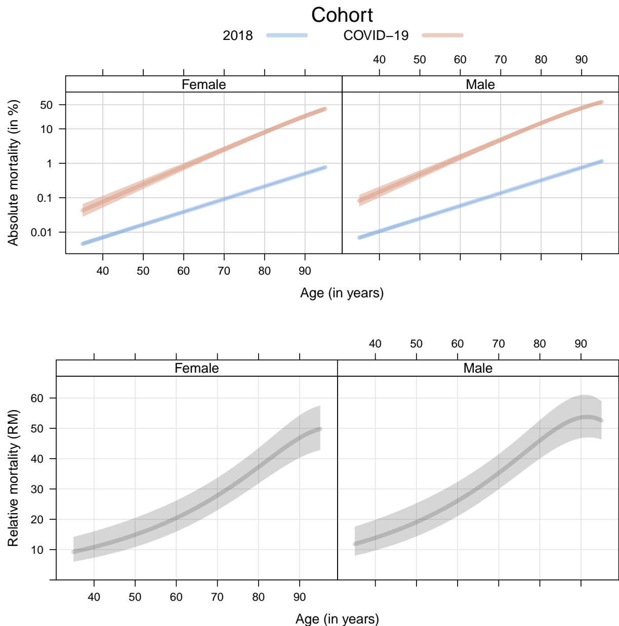
Figure 3: Swiss 2018 population and covid-19 cohorts. Comparison of absolute mortality (the probability of dying from any cause after 60 days, plotted on logarithmic scale) between the Swiss 2018 population and covid-19 cohorts, separately for females and males of different ages (top). Comparison of relative mortality (RM, the ratio of absolute mortalities in the covid-19 versus the 2018 cohort) between the two cohorts, for females and male of different ages (bottom). All estimates are plotted with 95% confidence bands.
