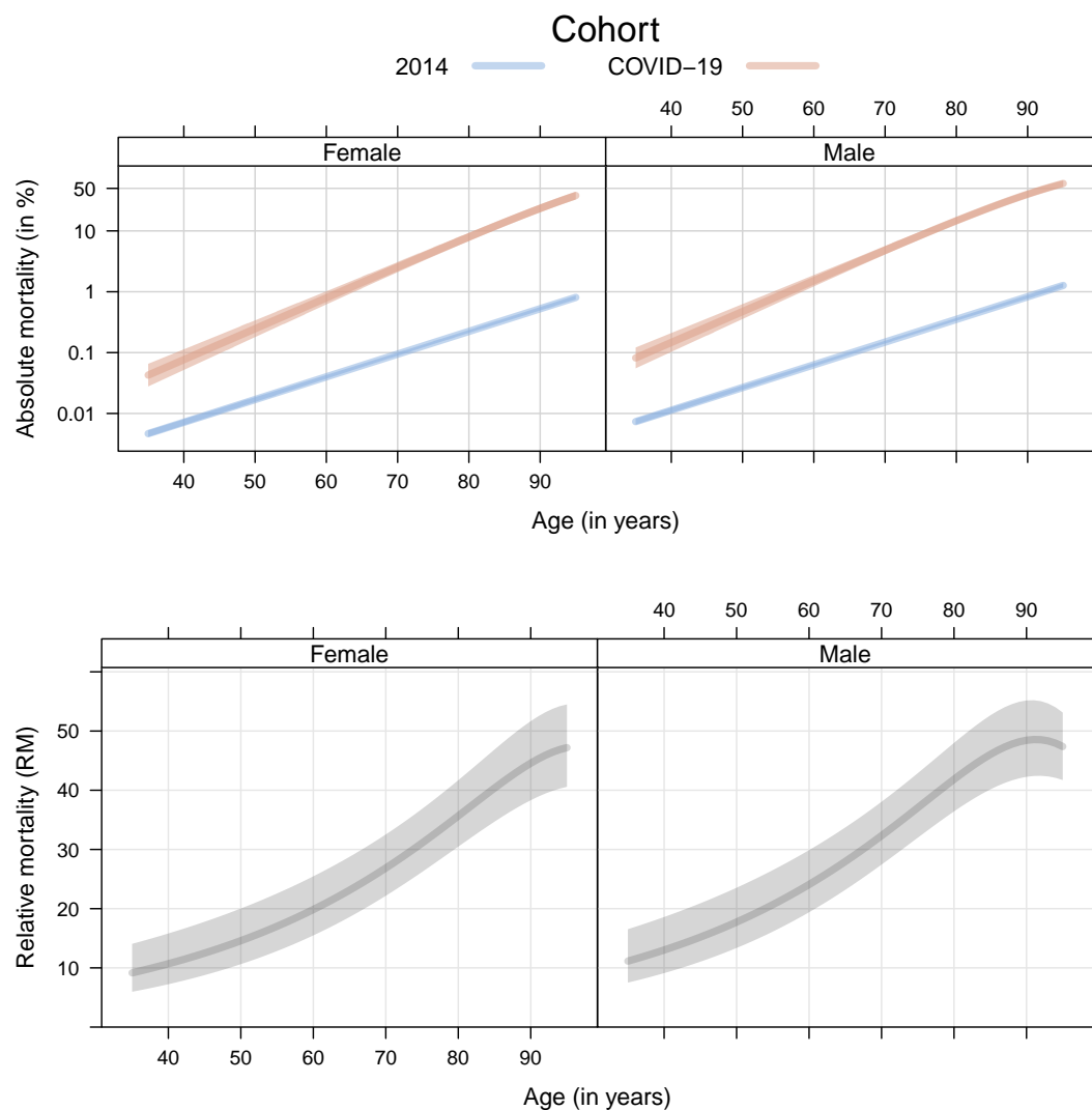
Supplementary Figure 10: Swiss 2014 population and covid-19 cohorts. Comparison of absolute mortality (the probability of dying from any cause after 60 days, plotted on logarithmic scale) between the Swiss 2014 population and covid-19 cohorts, separately for females and males of different ages (top). Comparison of relative mortality (RM, the ratio of absolute mortalities in the covid-19 versus the 2014 cohort) between the two cohorts, for females and male of different ages (bottom). All estimates are plotted with 95% confidence bands.
