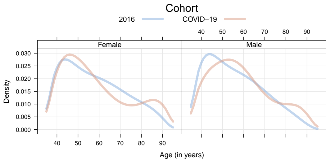
Supplementary Figure 5: Swiss 2016 population and covid-19 cohorts. Comparison of age densities between the Swiss 2016 population and covid-19 cohorts, separately for females and males.
