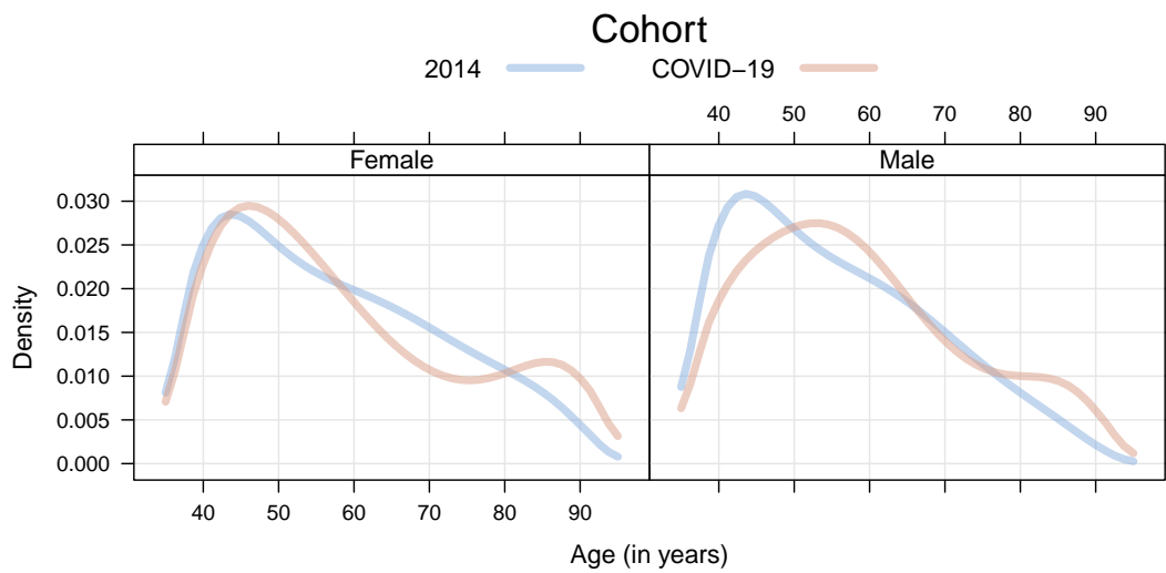
Supplementary Figure 9: Swiss 2014 population and covid-19 cohorts. Comparison of age densities between the Swiss 2014 population and covid-19 cohorts, separately for females and males.
