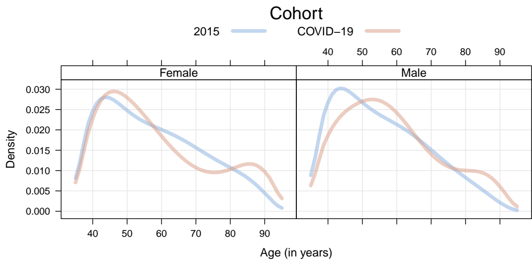
Supplementary Figure 7: Swiss 2015 population and covid-19 cohorts. Comparison of age densities between the Swiss 2015 population and covid-19 cohorts, separately for females and males.
