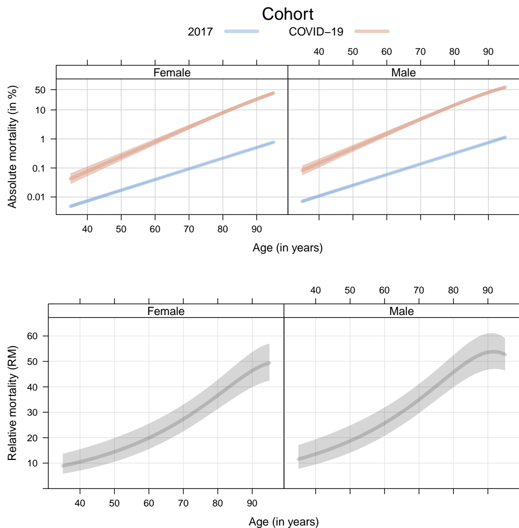
Supplementary Figure 4: Swiss 2017 population and covid-19 cohorts. Comparison of absolute mortality (the probability of dying from any cause after 60 days, plotted on logarithmic scale) between the Swiss 2017 population and covid-19 cohorts, separately for females and males of different ages (top). Comparison of relative mortality (RM, the ratio of absolute mortalities in the covid-19 versus the 2017 cohort) between the two cohorts, for females and male of different ages (bottom). All estimates are plotted with 95% confidence bands.
