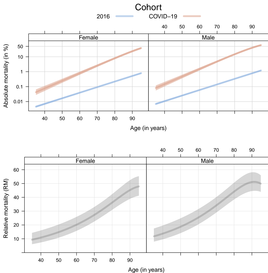
Supplementary Figure 6: Swiss 2016 population and covid-19 cohorts. Comparison of absolute mortality (the probability of dying from any cause after 60 days, plotted on logarithmic scale) between the Swiss 2016 population and covid-19 cohorts, separately for females and males of different ages (top). Comparison of relative mortality (RM, the ratio of absolute mortalities in the covid-19 versus the 2016 cohort) between the two cohorts, for females and male of different ages (bottom). All estimates are plotted with 95% confidence bands.
