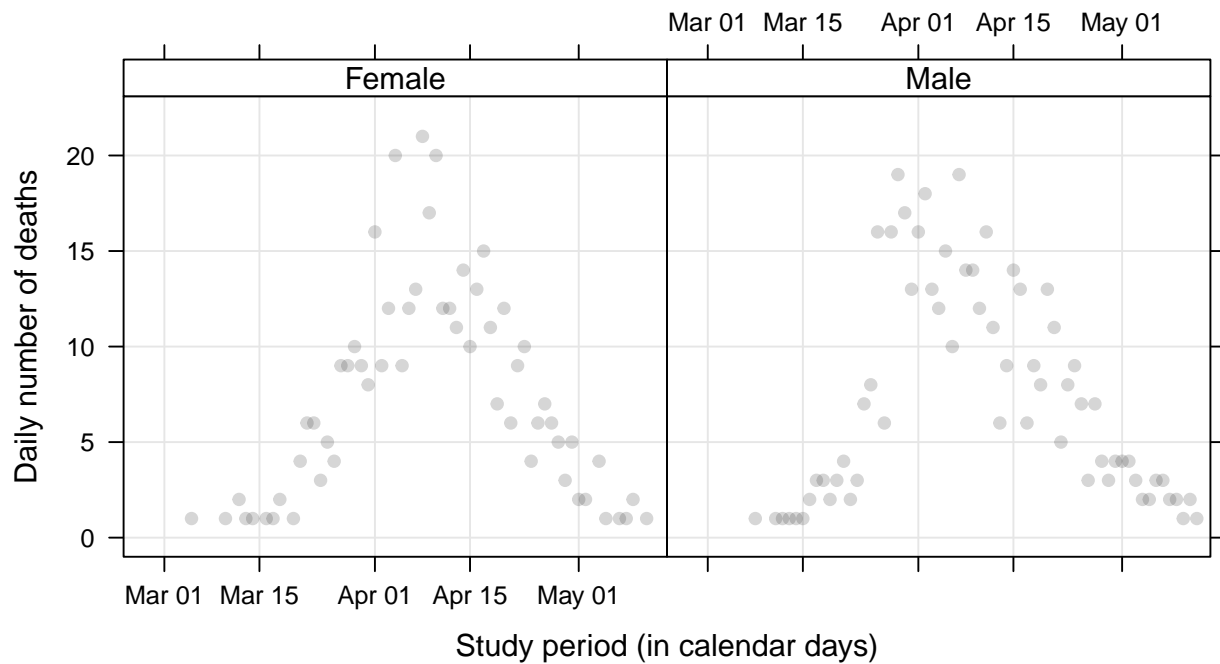
Figure 1: Swiss covid-19 cohort. Number of deaths from all causes reported between 2020-02-24 and 2020-05-14 in covid-19 patients (35 and 95 years old, not admitted to a hospital prior to testing, excluding post mortem tests).
