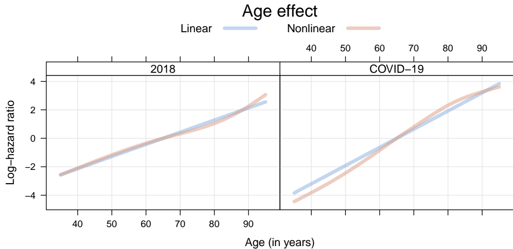
Supplementary Figure 1: Swiss 2018 population and covid-19 cohorts. Evaluation of linearity assumption on age. A Cox proportional hazards model was refitted allowing a nonlinear additive impact of age on the log-hazard function. The age effects of the linear Cox model, for females in the two study cohorts, are compared on the log-hazard ratio scale.
