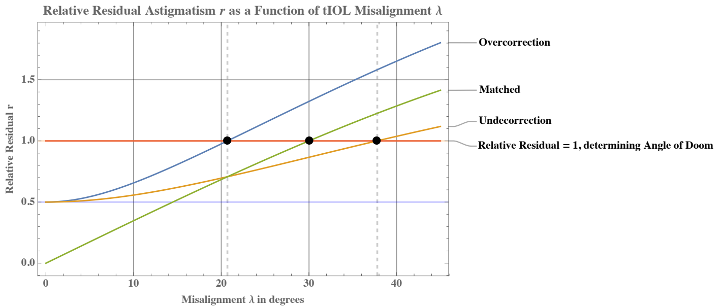
Figure 6 Relative residual error as a function of angle of misalignment for matched case (green) as well as over (blue) and undercorrection (orange). Angle of doom determined by intersection of each curve with r=1 . Observe that for undercorrection \Delta \sim 40 degrees and for overcorrection \Delta \sim 20 degrees.
