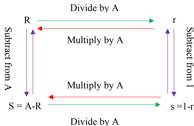
Figure 4 Navigating between 4 equivalent representations of residual astigmatism, 1) the full residual, R, 2) the fractional residual r, with respect to A, astigmatism to be corrected, 3) the magnitude of astigmatism having been corrected, S and 4) the fractional correction, s, with respect to A.
