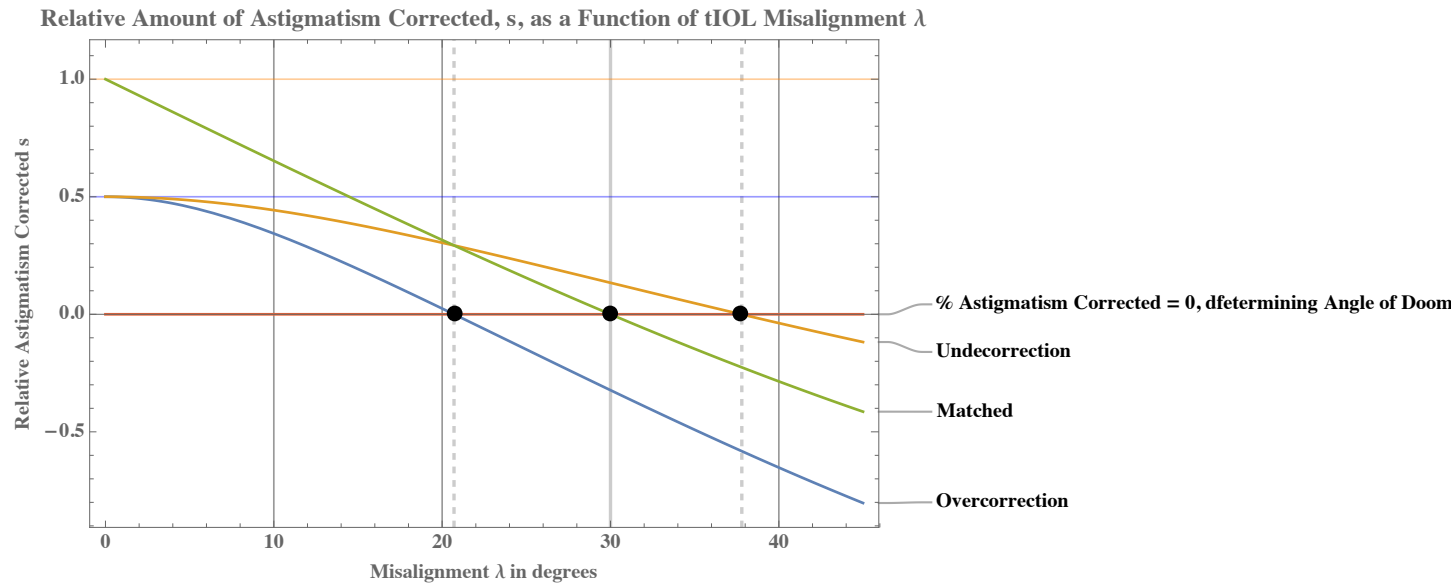
Figure 7 Relative amount of astigmatism corrected as a function of misalignment for matched case (green) as well as over (blue) and undercorrection (orange). Angle of doom determined by intersection of each curve with s=0 . Clearly here too we observe that for undercorrection \Delta \sim 40 degrees and for overcorrection \Delta \sim 20 degrees.
