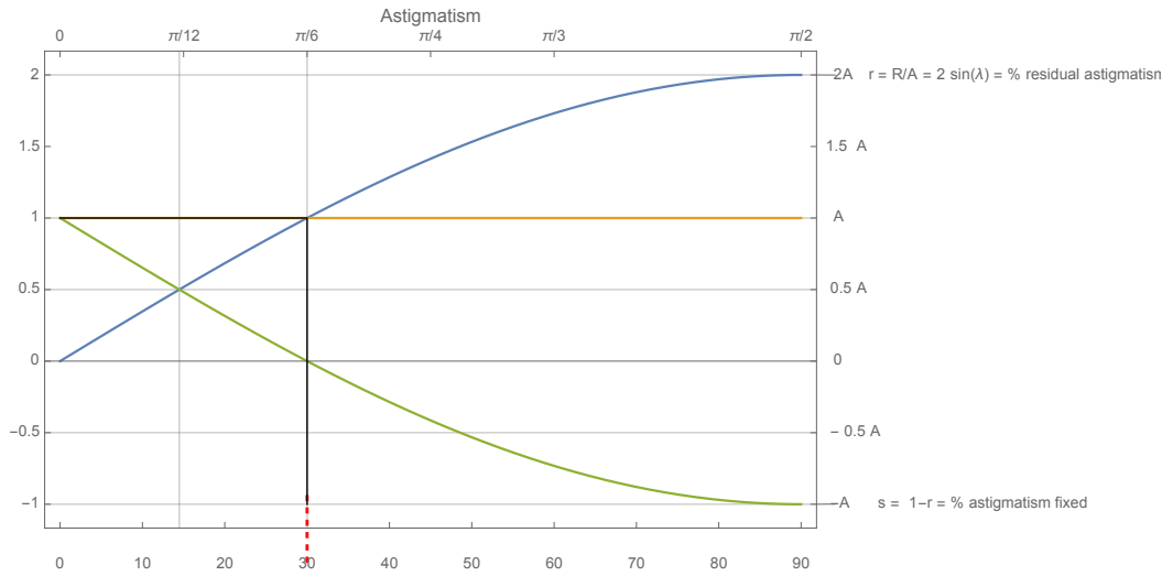
Figure 5 An astigmatism of cylinder value = A diopters, being corrected by a tIOL of L=A diopters as it rotates, results in residual astigmatism represented as magnitude of residual astigmatism (ascending curve), astigmatism corrected (descending curve) as full value of astigmatism (right scale) or its fractional representation wrt A (left scale).
