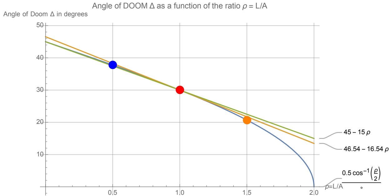
Figure 8 Angle of Doom \Delta as a function of \rho = \frac{L}{A} with linearization around (1,30)
