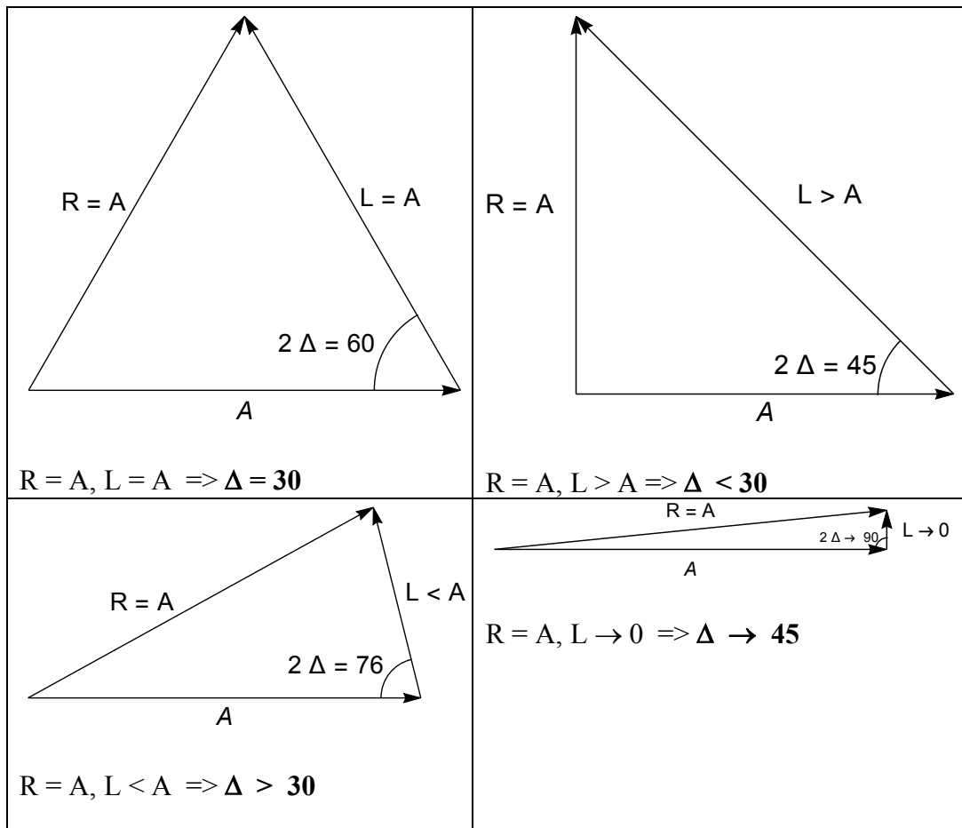
Figure 2 : Illustrates the cases of 1) perfect match of A and L resulting in an equilateral triangle and thus 2\Delta = 60 degrees and \Delta = 30 degrees, the “classical” result. 2) Overcorrection L \cong 1.4 A and \Delta = 22.5 and 3) Undercorrection L = 0.5 A and \lambda \cong 38 degrees. 4) Limit of “barely toric” IOL with \Delta \rightarrow 45 degrees.
