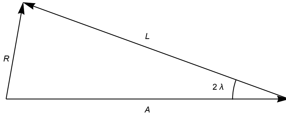
Figure 3. A triangle representation of astigmatism A with an attempted correction L that has rotated by an angle \lambda with respect to the intended meridian, with a residual astigmatism R . The geometric representation and residual calculation are based on a triangle with an angle 2\lambda between the sides, A and L . From elementary geometry an “SAS” (side angle side) triangle is uniquely determined and therefore both the residual astigmatism and its meridian are easily computable.
