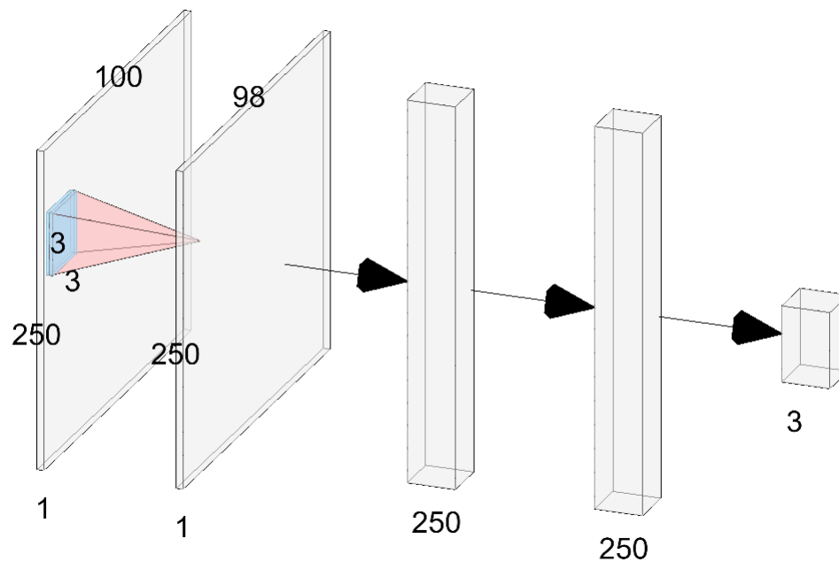
Figure 8. COVID-19 AI Network Architecture
