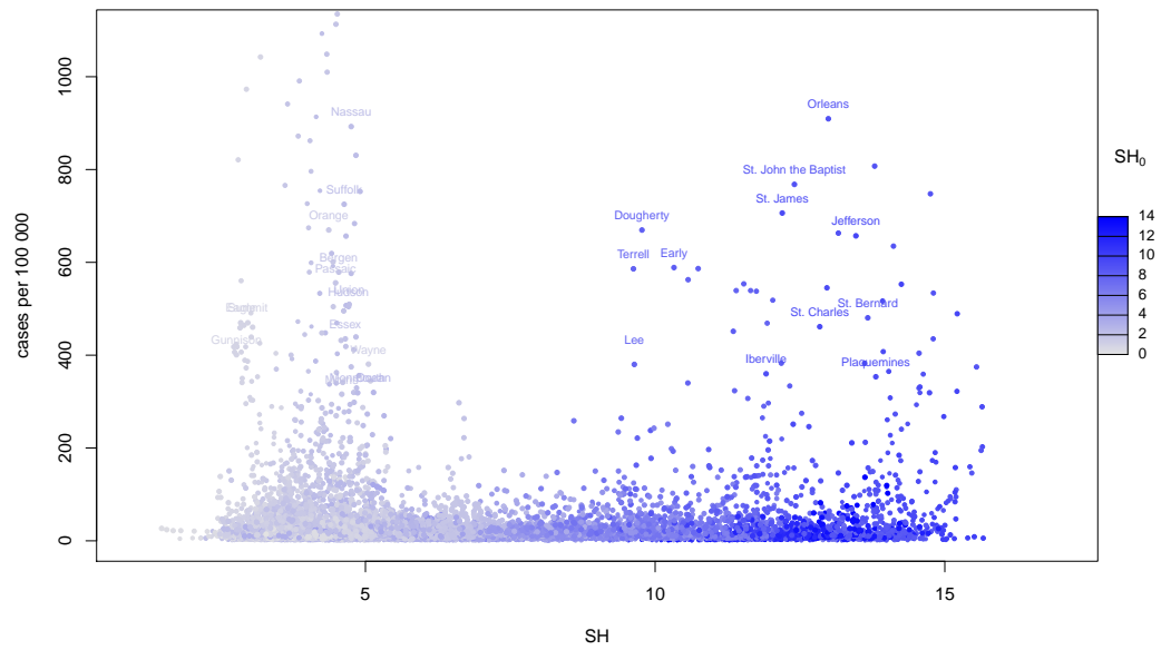
Fig 6. Evolution of cases in the USA and specific humidity. Cases per county in the USA against specific humidity. Dot colours are graded from grey to blue according to initial values of specific humidity (low to high), size of dots increase with time from the 20th of February to the seventh of April, between 10 days to two weeks after lockdown depending on State.
