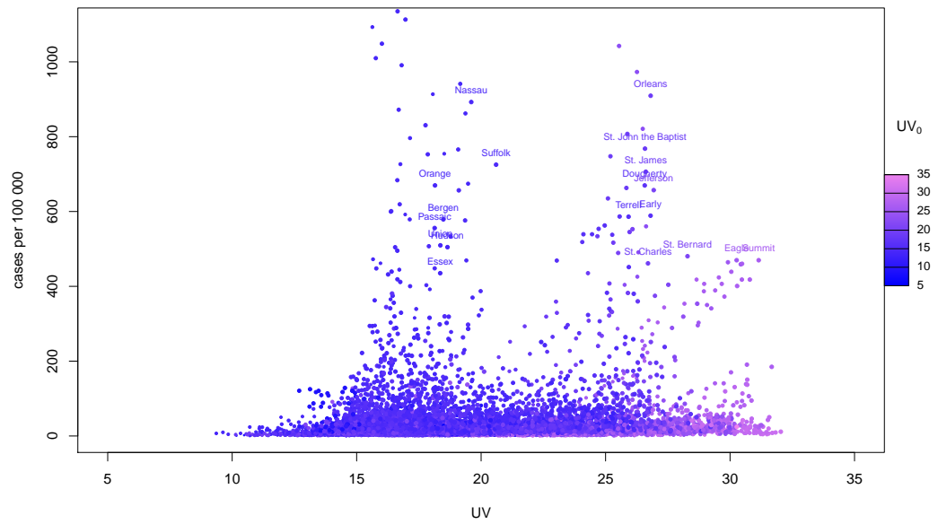
Fig 8. Evolution of cases in the USA and UV. Cases per county in the USA against ultraviolet radiation. Dot colours are graded from blue to violet according to initial values of ultraviolet radiation (low to high), size of dots increase with time from the 20th of February to the seventh of April, between 10 days to two weeks after lockdown depending on State.
