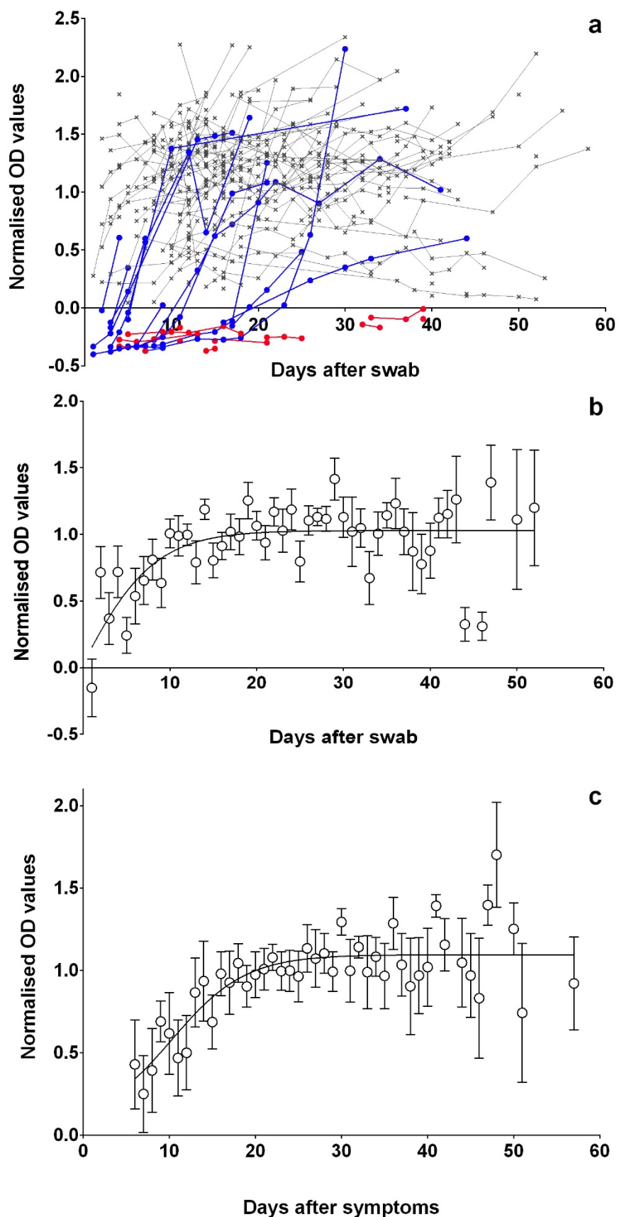
Fig. 1 Antibody dynamics
