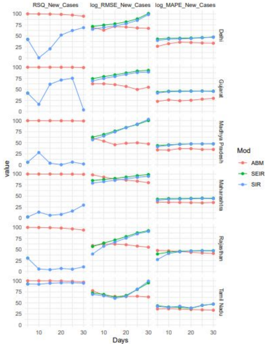
Figure 2 : Comparison of State-wise projection from different models, state-wise R -squared, log Root Mean Square Error of daily new cases from different models, log Mean Absolute Percentage Error of daily new cases from different models are shown in the plots above. (Log base 1.1 is taken to match the scales for plotting) (Plot shows evaluation for Delhi, Gujrat, Madhya Pradesh, Maharashtra, Rajasthan, Tamil Nadu)
