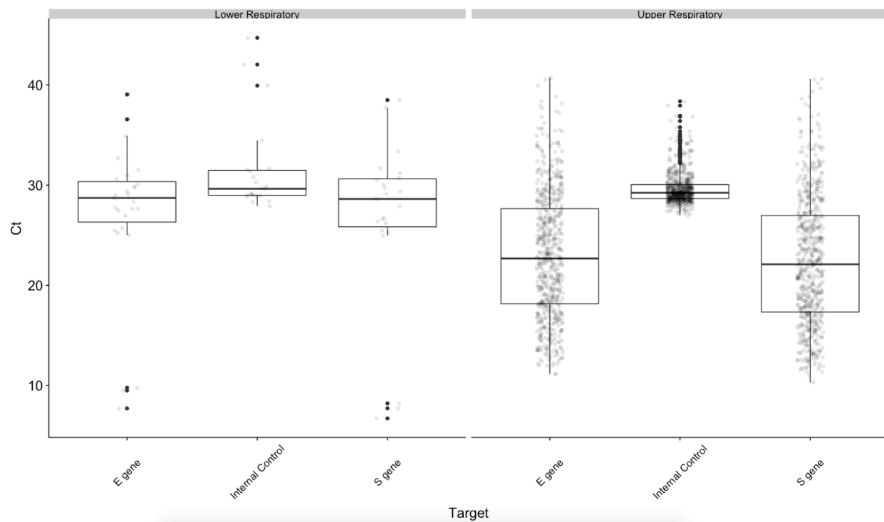
484 Figure 3. Distribution of Ct values for E gene, S gene, and Internal Control targets for all 485 upper respiratory tract (URT) and lower respiratory tract (LRT) specimens with detected 486 SARS-CoV-2. Mean Ct values between URT and LRT specimens were significantly 487 different for the E gene ( p=0.006 ) and S gene ( p=0.03 ) but not the I.C. ( p=0.7 ), though 488 the much smaller sample size for LRT is noted.
