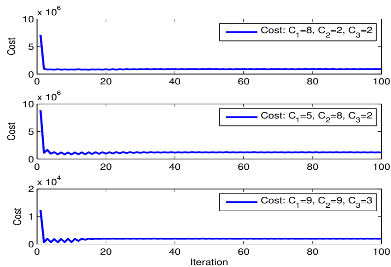
Fig. 12: The behavior of cost functional given in (12) with respect to iterations.
