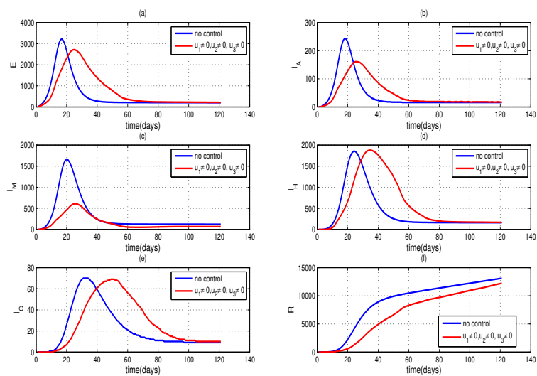
Fig. 6: The simulated solution curves for the Exposed (a), Asymptomatic (b), Symptomatic with mild (c), Isolated in hospitals (d), Treated in ICUs (e) and Recovered (f) for the optimal control problem given in (10)-(20) with A_1 = 50 , A_2 = 75 , A_3 = 60 , C_1 = 8 , C_2 = C_3 = 2 . It is assumed that the relative cost for social distancing and personal protection is high.
