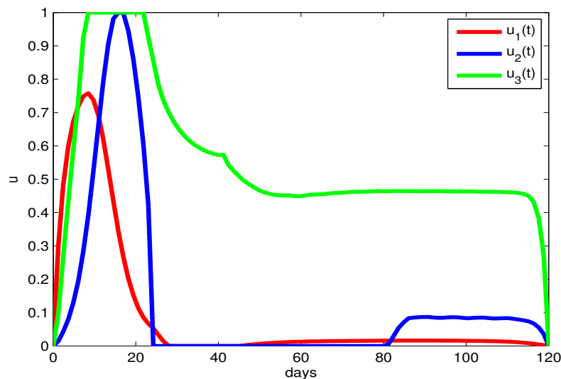
Fig. 9: The optimal control profiles u_1(t) , u_2(t) and u_3(t) with A_1 = 50 , A_2 = 75 , A_3 = 60 , C_1 = 5 , C_2 = 8 , C_3 = 2 .
