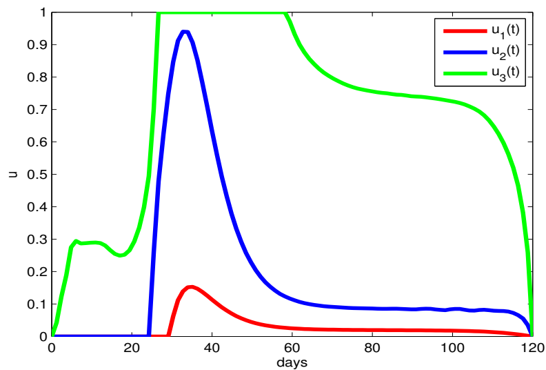
Fig. 11: The optimal control profiles u_1(t) , u_2(t) and u_3(t) with A_1 = 50 , A_2 = 75 , A_3 = 60 , C_1 = 9 , C_2 = 9 , C_3 = 3 .
