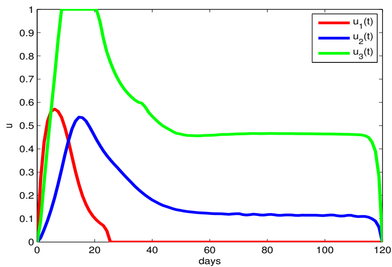
Fig. 7: The optimal control profiles u_1(t) , u_2(t) and u_3(t) with A_1 = 50 , A_2 = 75 , A_3 = 60 , C_1 = 8 , C_2 = C_3 = 2 .
