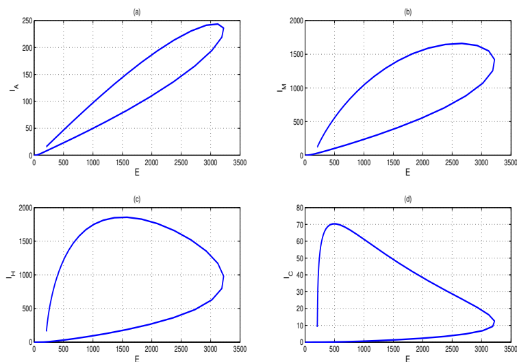
Fig. 4: Solution trajectories (E, I_A) , (E, I_M) , (E, I_H) and (E, I_C) for the problem 1 with fixed parameter \phi = 0.25 .
