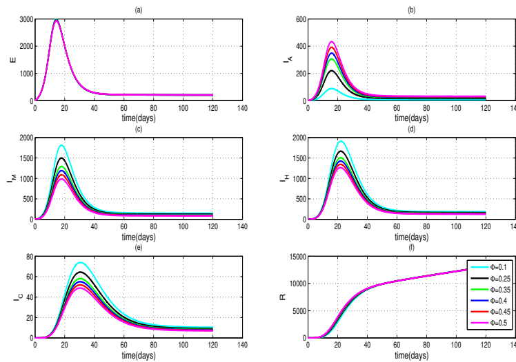
Fig. 3: The simulated solution curves for the Exposed (a), Asymptomatic (b), Symptomatic with mild (c), Isolated in hospitals (d), Treated in ICUs (e) and Recovered (f) as given in (1) with varying parameter \phi = (0.1, 0.25, 0.35, 0.4, 0.45, 0.5) .
