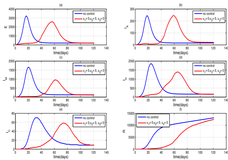
Fig. 10: The simulated solution curves for the Exposed (a), Asymptomatic (b), Symptomatic with mild (c), Isolated in hospitals (d), Treated in ICUs (e) and Recovered (f) for the optimal control problem given in (10)-(20) with A_1 = 50 , A_2 = 75 , A_3 = 60 , C_1 = 9 , C_2 = 9 , and C_3 = 3 . It is assumed that the relative cost for tracing and testing symptomatic cases is high while less importance is given for social distancing and personal protection.
