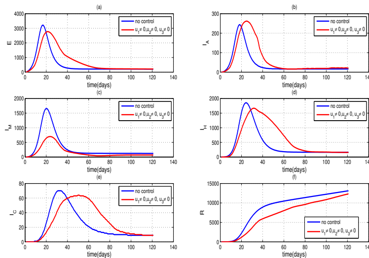
Fig. 8: The simulated solution curves for the Exposed (a), Asymptomatic (b), Symptomatic with mild (c), Isolated in hospitals (d), Treated in ICUs (e) and Recovered (f) for the optimal control problem given in (10)-(20) with A_1 = 50 , A_2 = 75 , A_3 = 60 , C_1 = 5 , C_2 = 8 , and C_3 = 2 . It is assumed that the relative cost for tracing and testing asymptomatic cases is high.
