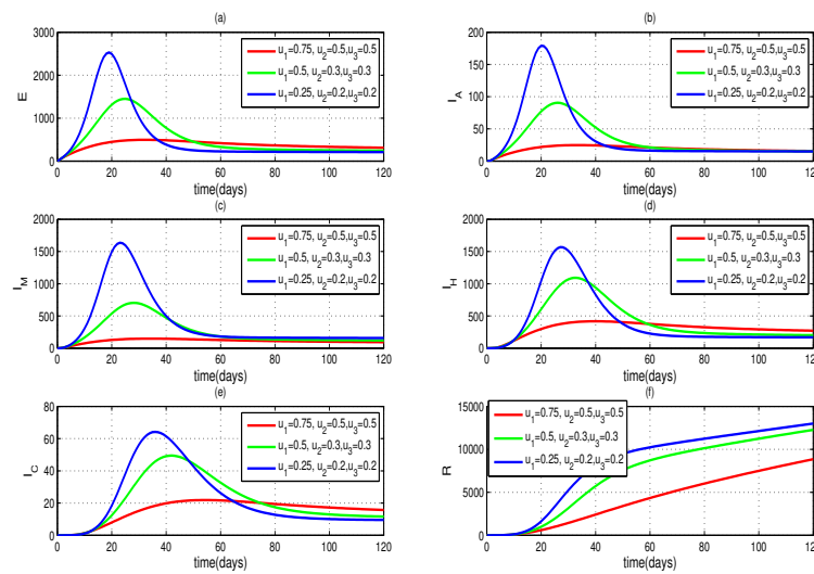
Fig. 5: The simulated solution curves for the Exposed (a), Asymptomatic (b), Symptomatic with mild (c), Isolated in hospitals (d), Treated in ICUs (e) and Recovered (f) as given in problem (10) considering combinations of non optimal control measures ( u_1 = 0.75, u_2 = 0.5, u_3 = 0.5 ), ( u_1 = 0.5, u_2 = 0.3, u_3 = 0.3 ) and ( u_1 = 0.25, u_2 = 0.2, u_3 = 0.2 ).
