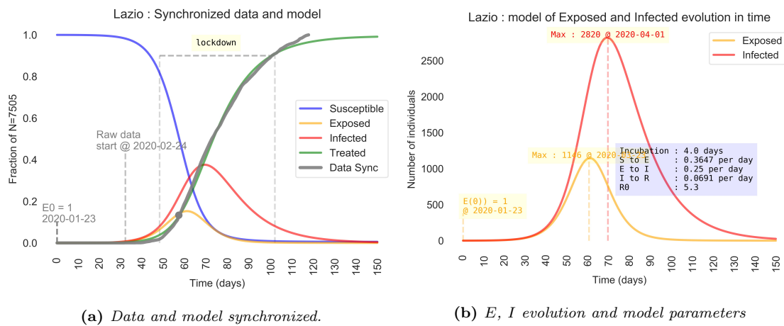
Figure 8: (a) The curve T of the model and T_{data} data has been synchronized at the point where the growth rate has been estimated. The ordinate scale is the ratio on the total number of cases N . (b) Detail of time evolution of E and I curves. The ordinate scale is the the number of individuals in the compartments E, I .
