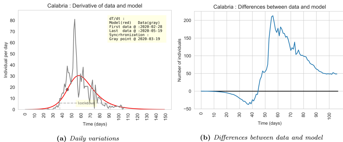
Figure 13: (a) Daily variation of T_{data} and of the T model (red). (b) Differences between T_{data} and the model T .
