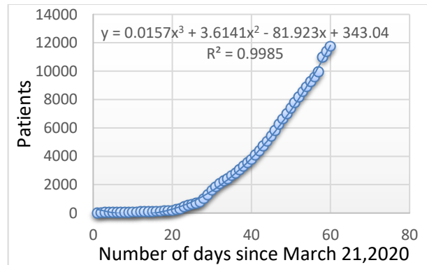
Figure 4: Polynomial regression model analysis for few representative states: (a) Total number of cases as a function of training data set since March 21, 2020. (b) Total number of cases as a function of test data from May 08, 2020 to May 19, 2020. Predicted patients from May 20, 2020 to June 02, 2020 are also plotted.
