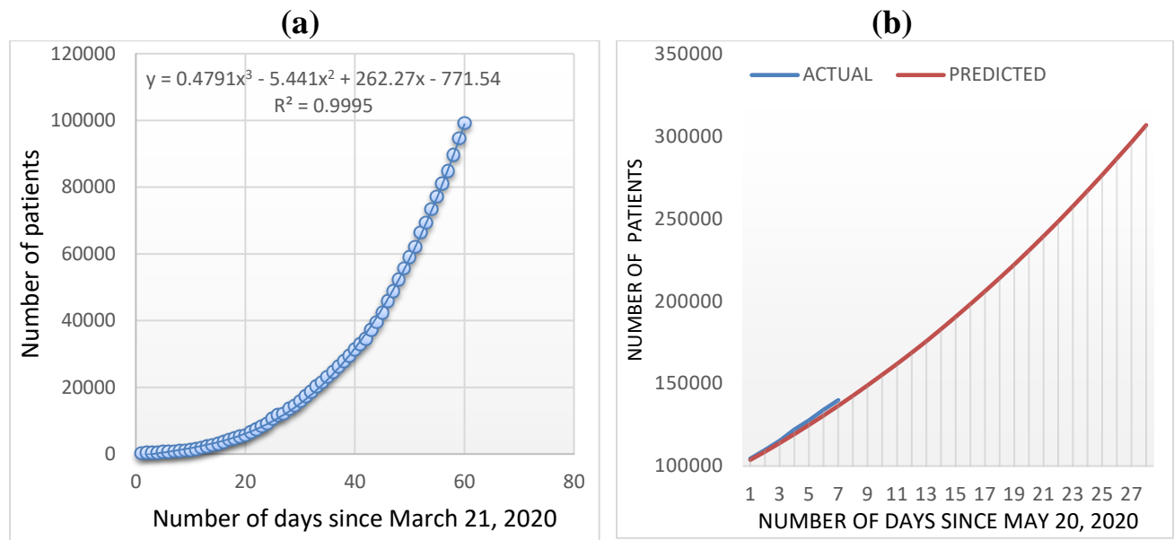
Figure 3: Polynomial regression model analysis for India. (a) Total number of cases as a function of training data set since March 21, 2020. (b) Total number of cases with test data from May 20, 2020 to May 26, 2020. Predicted patients from May 27, 2020 to June 16, 2020 are also plotted.
