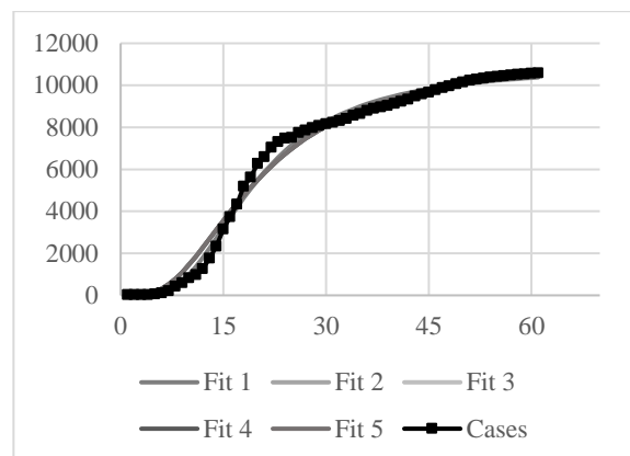
Figure 3. Five Log-logistics fit compared to South Korea confirmed cases
