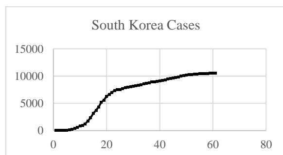
Figure 1. South Korea SARS-CoV-2 total cases
