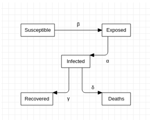
Figure 3: SEIRD Model
