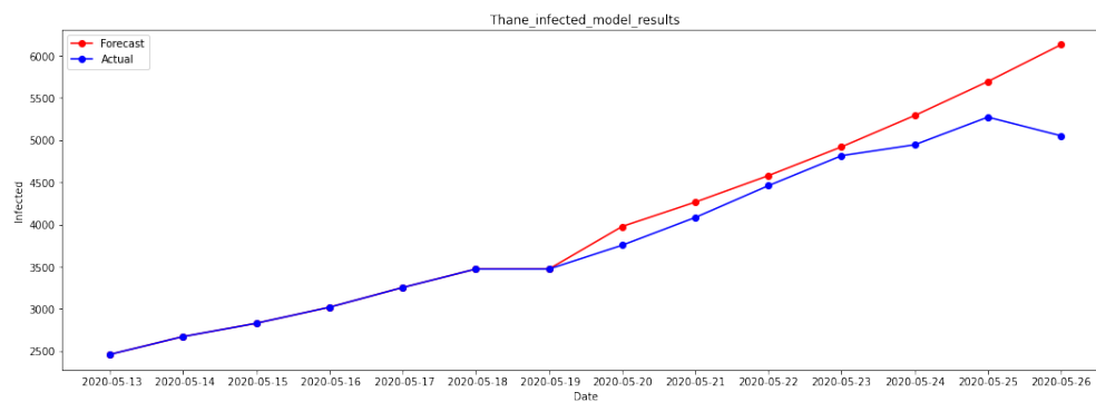
Figure 19: Plots for Actual vs Forecasted Infected Cases for Thane on Test Data; MAPE 7.36%
