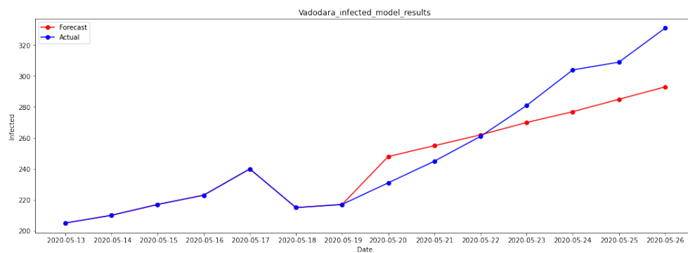
Figure 25: Plots for Actual vs Forecasted Infected Cases for Vadodara ; MAPE 6.25%
