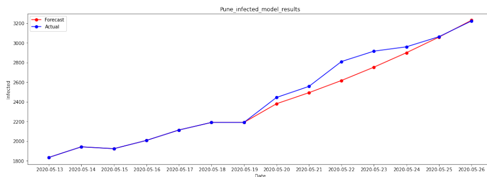
Figure 21: Plots for Actual vs Forecasted Infected Cases for Pune ; MAPE 2.85%
