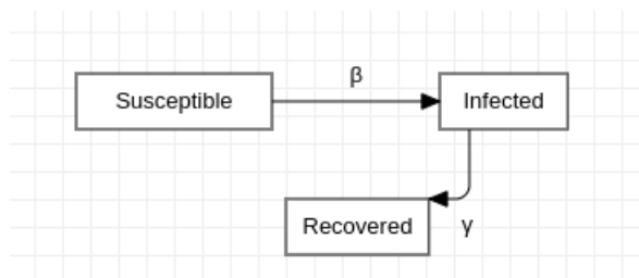
Figure 1: SIR Model.
