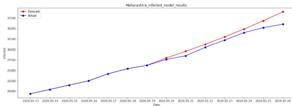
Figure 13: Plots for Actual vs Forecasted Infected Cases for Maharashtra ; MAPE 3.60%
