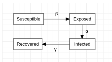
Figure 2: SEIR Model
