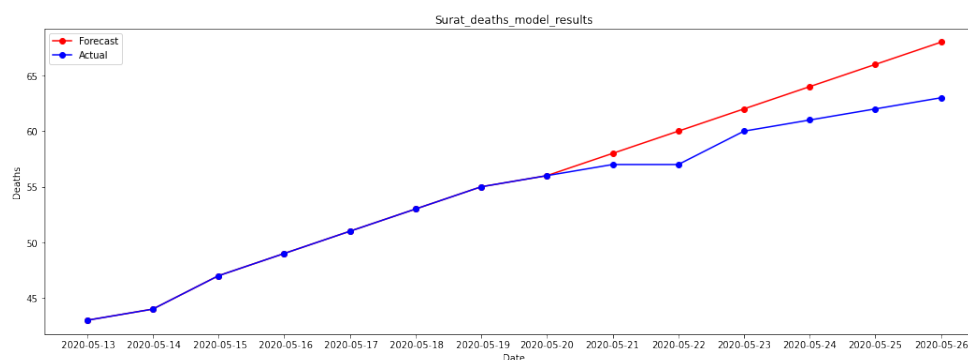
Figure 28: Plots for Actual vs Forecasted Death Cases for Surat ; MAPE 4.23%
