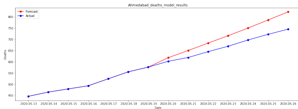
Figure 24: Plots for Actual vs Forecasted Death Cases for Ahmedabad ; MAPE 6.76%
