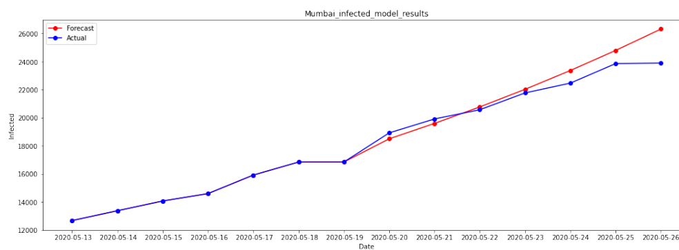
Figure 17: Plots for Actual vs Forecasted Infected Cases for Mumbai ; MAPE 3.43%
