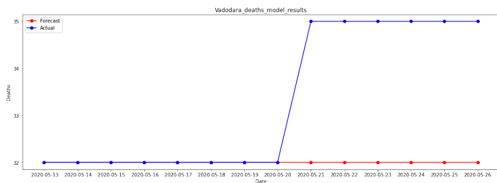
Figure 26: Plots for Actual vs Forecasted Death Cases for Vadodara ; MAPE 7.34%
