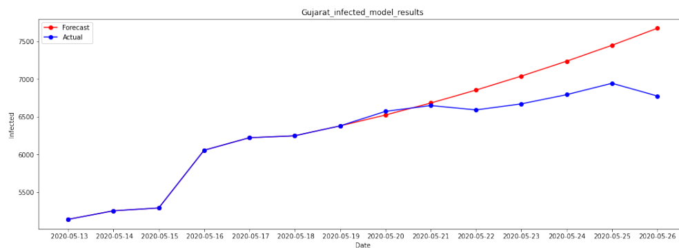
Figure 15: Plots for Actual vs Forecasted Infected Cases for Gujarat ; MAPE 5.39%
