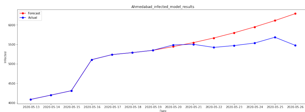
Figure 23: Plots for Actual vs Forecasted Infected Cases for Ahmedabad ; MAPE 5.98%
