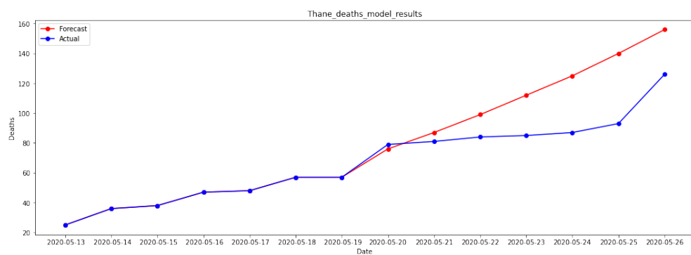
Figure 20: Plots for Actual vs Forecasted Death Cases for Thane ; MAPE 25.55%
