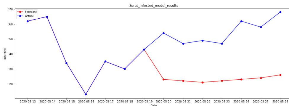
Figure 27: Plots for Actual vs Forecasted Infected Cases for Surat ; MAPE 8.98%
