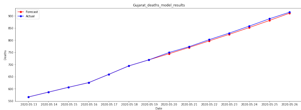
Figure 16: Plots for Actual vs Forecasted Death Cases for Gujarat ; MAPE 0.6%
