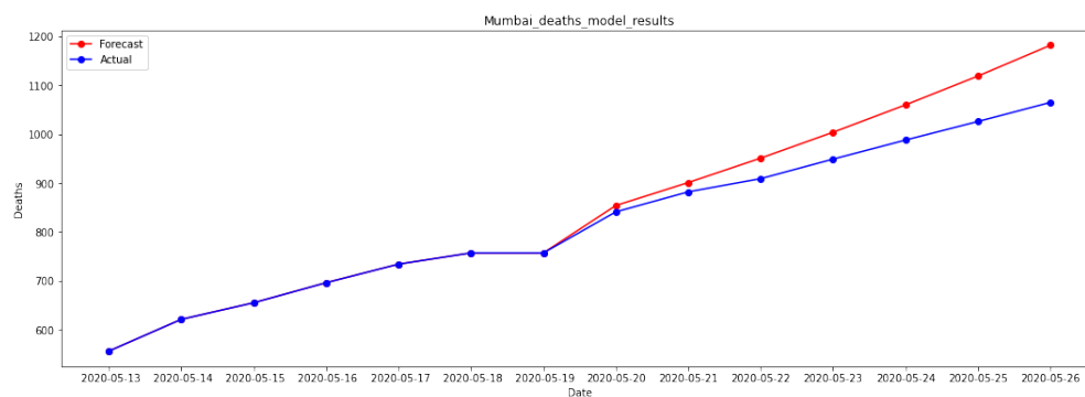
Figure 18: Plots for Actual vs Forecasted Death Cases for Mumbai ; MAPE 5.92%
