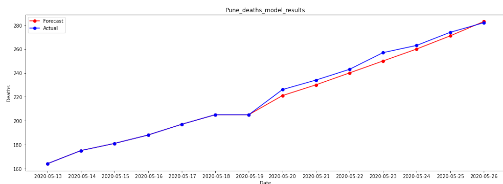
Figure 22: Plots for Actual vs Forecasted Death Cases for Pune on Test Data; MAPE 1.49%
