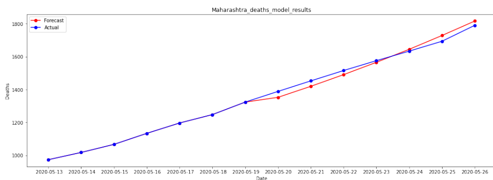
Figure 14: Plots for Actual vs Forecasted Death Cases for Maharashtra ; MAPE 1.61%
