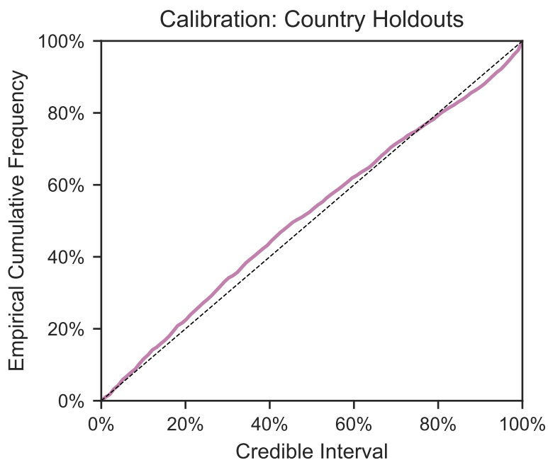
Figure C.23: Calibration in held-out countries with leave-one-out cross-validation. Here we include only those 35 countries that were not used to select the hyperparameter. We show the first 14 days of cases and deaths in each country and then extrapolate to future days within the period of analysis. The plot shows the percentage of observed daily case and death counts that lie within the X% credible interval, across all countries and days.
