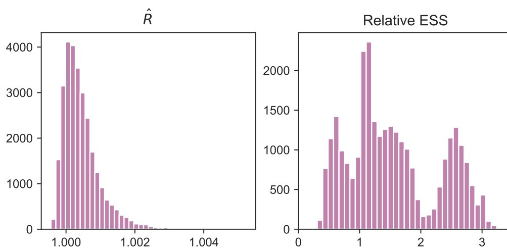
Figure C.24: MCMC stability results. Left : R-hat statistic. Values are close to 1, indicating convergence. Right : Relative effective sample size. A value of 1 indicates perfect decorrelation between samples. Values above (below) 1 indicate that the effective number of samples is higher (lower) than the actual number of samples due to negative (positive) correlation, respectively.
