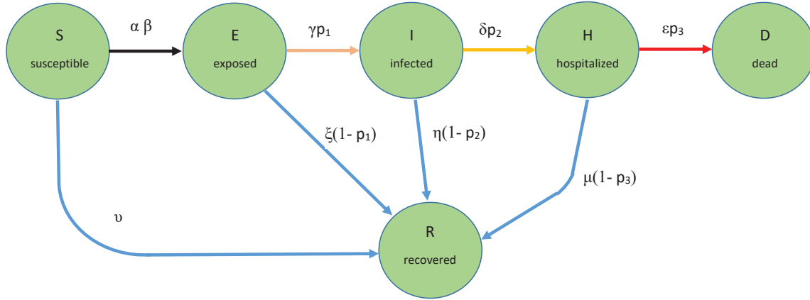
Figure 1: Rate processes that describes the progress between the groups in the SEIHRD model.
