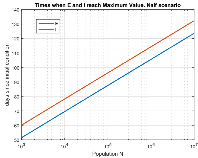
Figure 4: Times when Exposed and Infected groups reach Maximum Values. Naif Scenario
