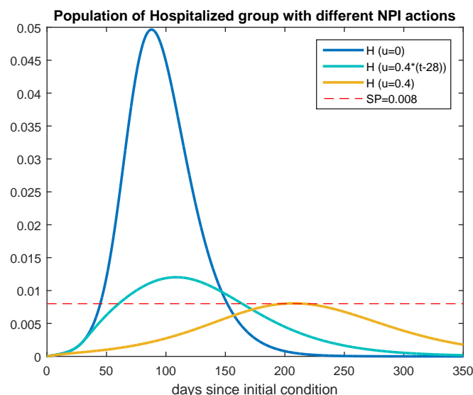
Figure 6: Population of Hospitalized group with no NPI (blue), with a NPI of 40% effectiveness (yellow), with an intervention of 40% effectiveness applied 4 weeks after the appearance of the first case (light blue) and SP (red). \beta = \alpha/2
