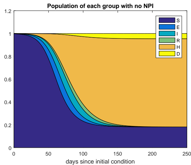
Figure 5: Population of each group with no NPI. \beta = \alpha/2
