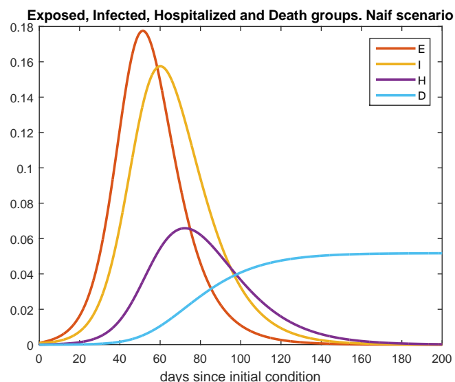
Figure 3: Population of Exposed, Infected, Hospitalized and Deaths group with no NPI. Naif Scenario
