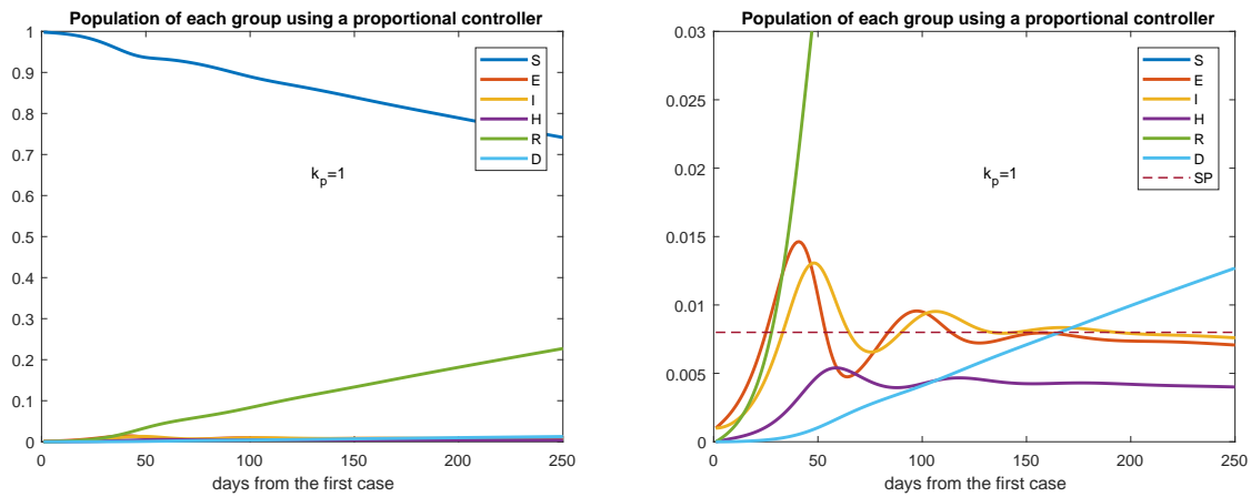
Figure 7: Evolution of every group over time with a proportional control action with gain k_p = 1 (left). The picture at the right is a zoom of that at the left. Set point equal to 0.008.
