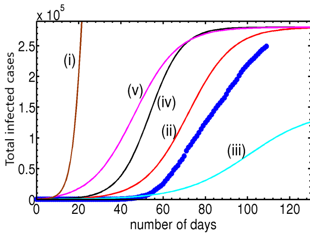
FIG. 1. (Color online) Plots for the total infected population N_t for decreasing values of N_a(0) as a function of time (in days) : (i) N_a(0) = 8 \times 10^5 , (ii) 2.8 \times 10^5 , and (iii) 1.45 \times 10^5 respectively, keeping f_i p_i \beta_i = 3.3913 \times 10^{-7} and \alpha_s p_s = 1.0 \times 10^{-4} fixed. The curve (ii) shows decreasing N_a(0) by a factor of 5.51 leads to slow increase in N_t . (iv) Plot of N_t for f_i p_i \beta_i = 4.752 \times 10^{-7} , keeping N_a(0) = 2.8 \times 10^5 and \alpha_s p_s = 1.0 \times 10^{-4} . Smaller values of f_i p_i \beta_i take longer time for N_t to grow as is clear. See (ii) and (iv). (v) Plot of N_t for \alpha_s p_s = 1.1 \times 10^{-3} , keeping N_a(0) = 2.8 \times 10^5 and f_i p_i \beta_i = 3.3913 \times 10^{-7} fixed. Increase in \alpha_s p_s leads to a faster initial growth seen in (v) and (iii). Also show is the cumulative number of infections (●) for the UK.
