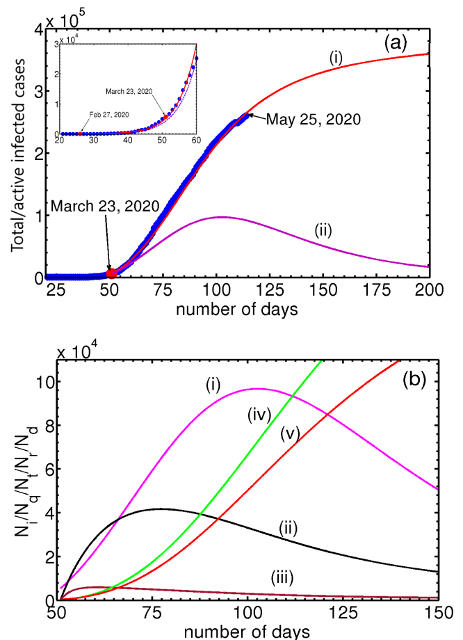
FIG. 4. (a) Inset: Plot of the total infected population (continuous curve), along with the UK data \bullet from February 27, 2020 till March 31. Also shown is the active infected N_i (dotted curve). Post Lock-down period: Plots of the total infected population (curve marked i) along with the corresponding data for the UK \bullet from March 23, 2020. Curve marked (ii) shows the active infected. (b) Plots of the infected (i), quarantined (ii), traced (iii), recovered (iv) and deceased (v), starting from March 23, 2020. The values of \alpha_s p_s = 2.9 \times 10^{-3} , \alpha_s p_q = 1.15 \times 10^{-2} and \alpha_t p_t = 5.8 \times 10^{-3} Other parameter values are the same as given in Table I.
