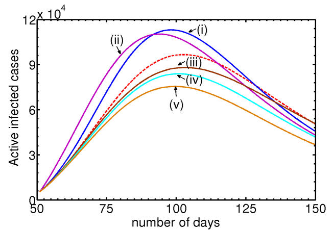
FIG. 3. (Color online) Calibration of parameters for identifying the relative importance of transitions contributing to N_i by varying one parameter, keeping all others parameters fixed at reference values listed in Table I. The dotted curve is the reference plot for the active infected population N_i corresponding to the values in the Table I. (i) Plot of N_i for a 20% increase in f_i p_i \beta_i , showing a shift and increased peak height. (ii) Similar effect is observed when \alpha_s p_s is increased by a factor 2. (iii) Decrease in the peak height when \alpha_s p_q is increased. (iv) Peak height decreases as \kappa_d is increased by 30%. (v) Similar effect is seen when the recovery rate is increased.
