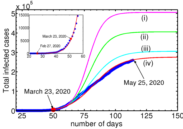
FIG. 2. Figure shows the two-phase evolution of the disease. The inset shows the good fit using Eq. (17) with the cumulative infected cases for the UK • prior to March 23, 2020. Parameter values used are N_a(0) = 1.86 \times 10^5 , N_t(0) = 13 , \alpha_c p_c = 9.0 \times 10^{-6} , f_i p_i \beta_i = 1.205 \times 10^{-6} . Post lock-down period: The four curves (i-iv) correspond to the four iterations of N_a(0) values. (i) N_a(0) = 5.0 \times 10^5 , \alpha_s p_s = 0.0 , (ii) N_a(0) = 4.0 \times 10^5 , \alpha_s p_s = 1 \times 10^{-3} , (iii) N_a(0) = 3.0 \times 10^5 , \alpha_s p_s = 2.8 \times 10^{-3} , and (iv) N_a(0) = 2.70 \times 10^5 , \alpha_s p_s = 2.8 \times 10^{-3} . The initial value of N_t(0) = 5687 on March 23, 2020.
