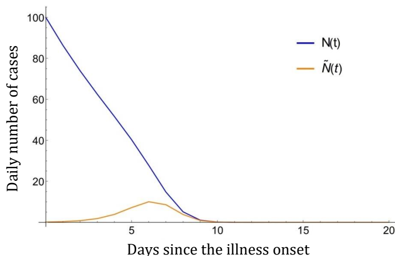
Figure 4: The graphs show the behavior of the number of infected cases N(t) (blue) and detected cases \tilde{N}(t) (orange) in function of time
