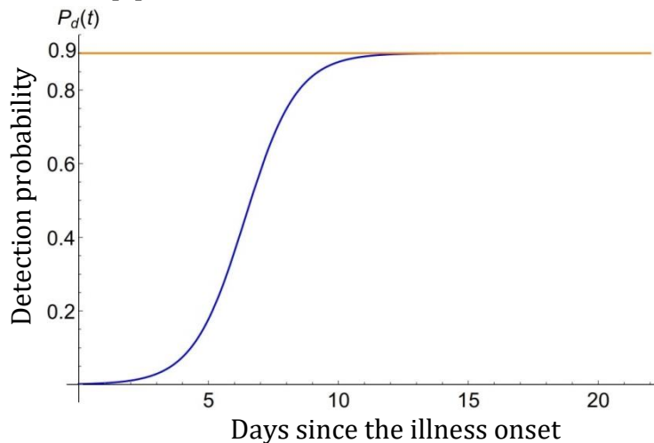
Figure 3: Graphic illustrating the behavior of the P_d(t) CDF by considering M=90\% and \delta_0 = 6.4 days
