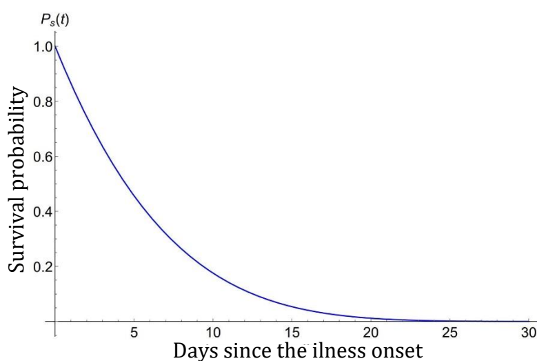
Figure 1: The behavior of P_s(t) function
