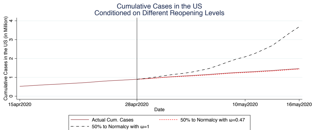
Figure A3. Out-of-Sample Prediction with the Standard SIR Model. The vertical line indicates the last day of our data sample.
