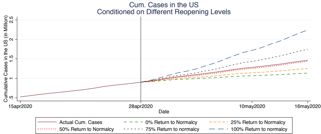
Figure 1. Out-of-Sample Prediction under Different Reopening Strategies. The vertical line indicates the last day of our data sample.
