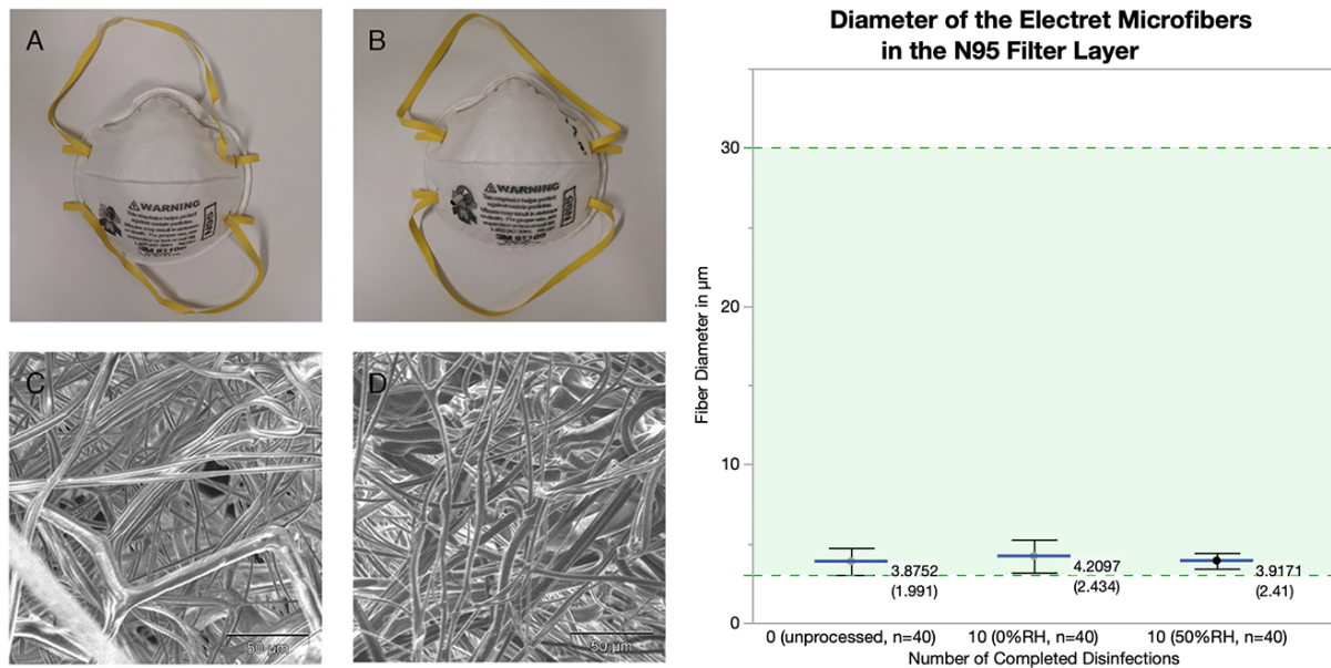
Figure 2: The effect of thermal disinfection on the structural properties of N95 respirators. (Left) The macroscopic and microscopic integrity of the respirator is preserved after repetitive disinfection. The upper left panels compare new (A) to ten times disinfected N95 respirators (B). Panels C and D show their filter layer in 650x magnification (SEM Image, Scale bar 50 \mu\text{m} , type 8110s, 3M, Minnesota, USA). (Right): Shown is the fiber diameter of unprocessed and ten times disinfected N95 filters (0% and 50%RH), with the typical fiber diameter range of 3M N95 filters highlighted in green (9). Shown are the mean fiber diameters with 99% confidence intervals as error bars. Graphs are labelled with mean \pm SD.
