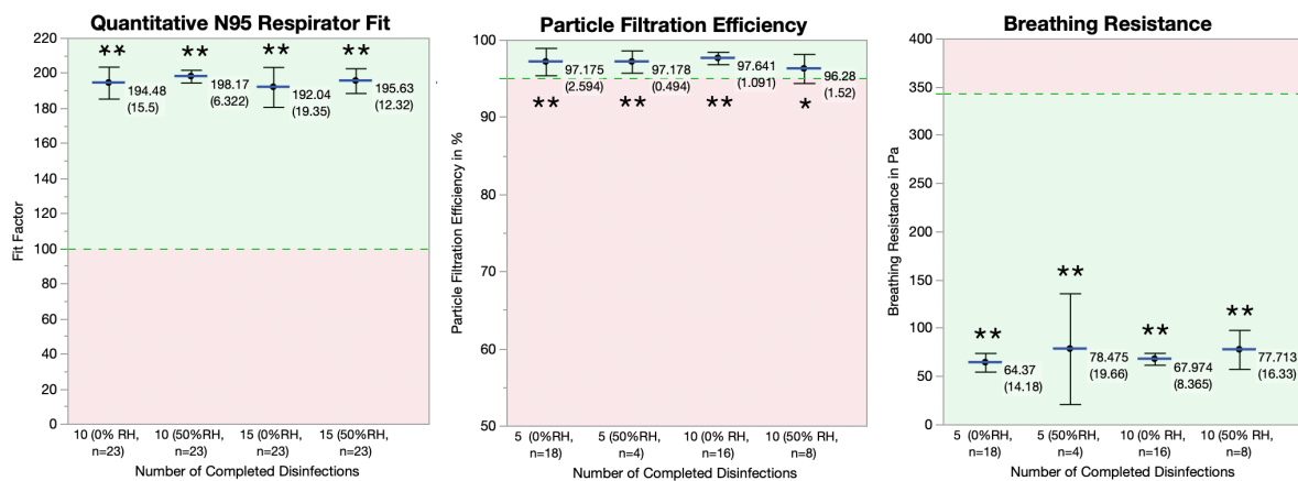
Figure 3: Function of thermally disinfected N95 respirators. Shown are the quantitative fit factors (left), particle filtration efficiency (centre) and breathing resistance (right) of thermally disinfected N95 respirators (0% and 50% RH). The US-governmental pass values for each test are indicated by a dashed line (11, 15, 16). Graphs are displayed as means with 99% confidence intervals and labelled with the mean \pm SD. Groups that significantly exceeded the pass value are labelled with a double asterisk (** p < 0.01 ; * p = 0.024 ).
