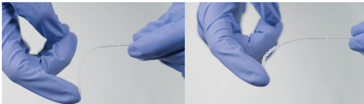
Figure 4: Comparison of bending modes for Generation 1 (Left) and Generation 2 (Right) latticed NP swabs. When force is applied to the tip of the swab, Generation 1 reacts by bending the most in the neck, below the bulb. In Generation 2, the bending is concentrated in the swab bulb.
