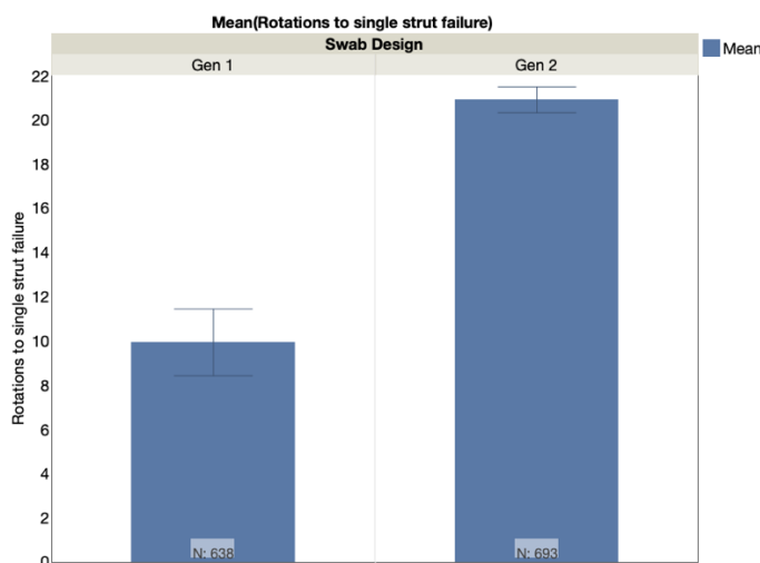
Figure 2: In process validation, a large number (>600) of samples were tested in simulated use models. The samples were monitored carefully for the first sign of a single strut failure. Compared to Generation 1 swabs, Generation 2 swabs were able to withstand almost double the turns until the first strut failure.
