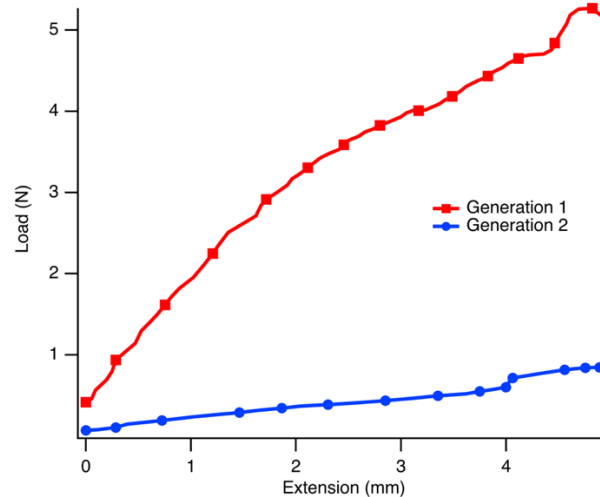
Figure 3: Comparison of Generation 1 and Generation 2 latticed NP swabs in the three-point bend force measurement test. Generation 2 requires less force to deflect, which allows it to navigate the nasal passageway with less force.
