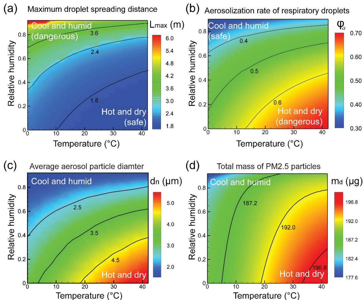
Figure 2. Effect of environmental factors on the transmission of COVID-19 via means of droplets contact and exposure to aerosol particles, respectively. (a) The maximum droplet traveling distance L_{\max} under different weather conditions in terms of temperature and relative humidity. Droplets can reach a longer distance in a cool and humid environment. (b) Aerosolization rate \phi_a , defined as the percentage of respiratory droplets turning into aerosol particles that can potentially travel beyond L_{\max} , under different weather conditions in terms of temperature and humidity. (c) The average diameter of completely dry aerosol particles, under different weather conditions. (d) The total mass of PM 2.5 floating in air that are produced by respiratory droplets per person at steady state in an enclosed space.
