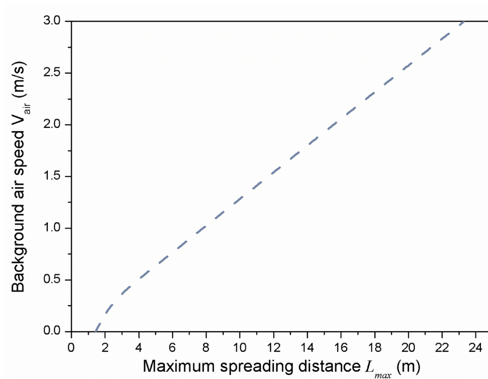
Figure 3. The effect of a horizontal, constant background airflow. Droplet spreading distance L_{max} as a function of a horizontal, constant air speed.
